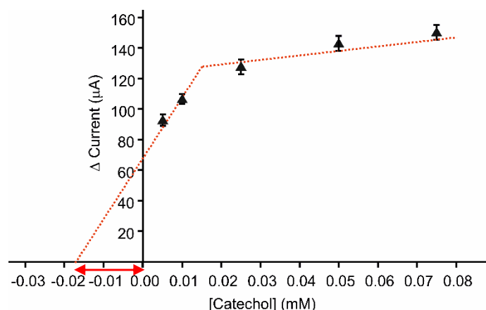
Figure 6: Calibration curves to increasing concentrations of catechol of the CS-MIP/BDD sensor in a diluted wine sample (10% diluted in 0.1M PBS solution, pH 7.4). ↔ Original concentration of catechol in diluted wine.
