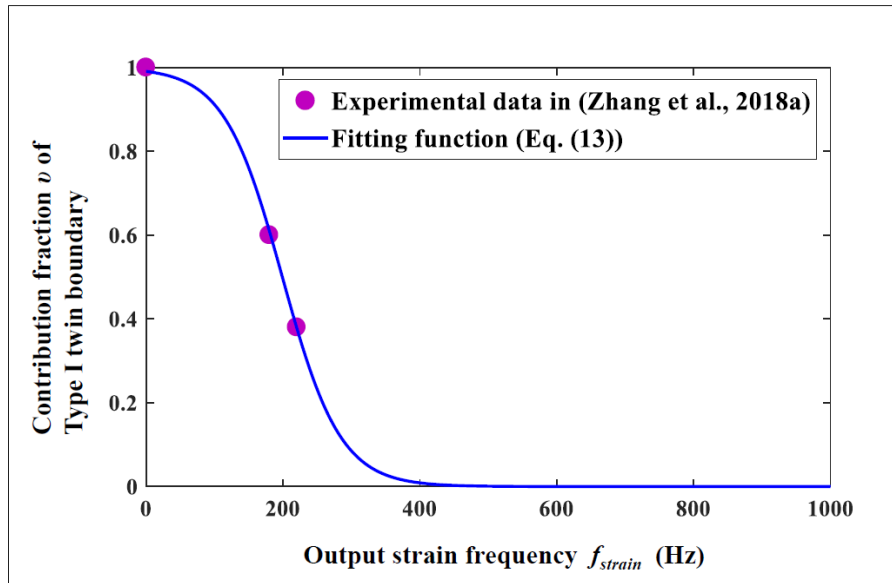
Fig. 3. Contribution fraction v of Type I twin boundary at different levels of output strain frequency f_{strain} .
