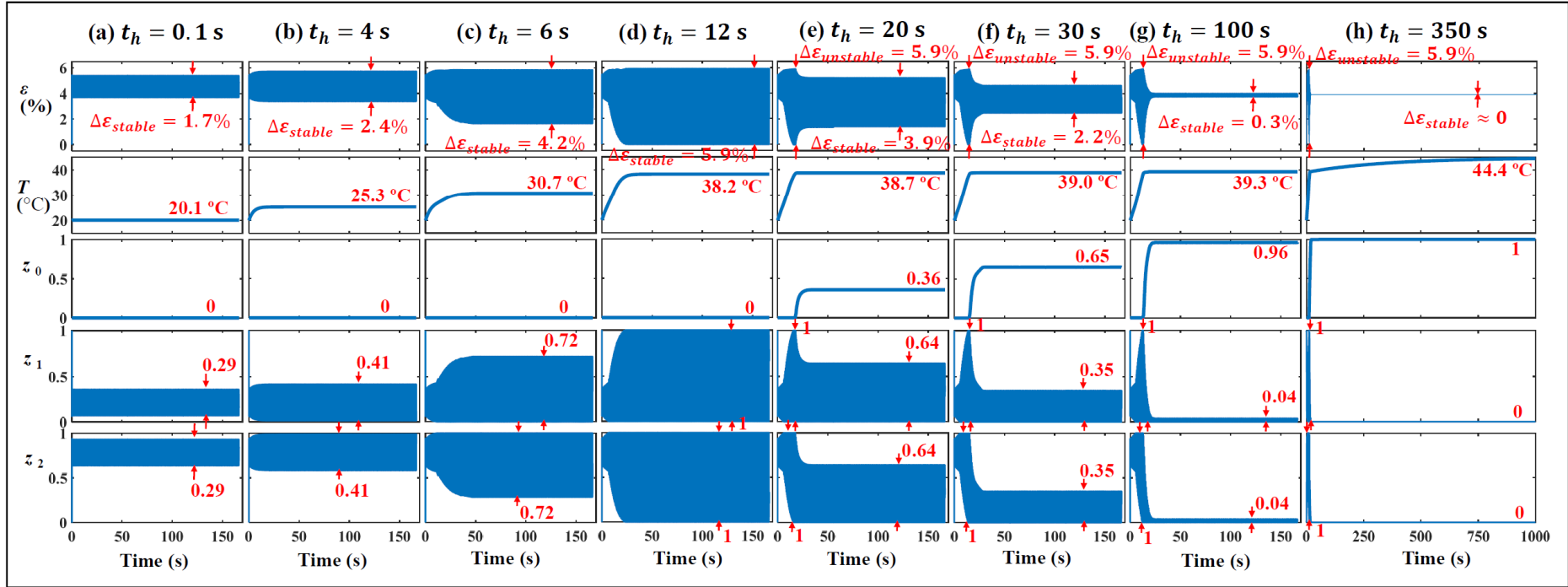
Fig. 9. The simulated evolutions of strain \epsilon , temperature T , volume fraction z_0 of austenite, volume fraction z_1 of martensite variant 1 and volume fraction z_2 of martensite variant 2 under different ambient heat exchange conditions. The characteristic ambient heat-transfer time t_h changes from 0.1 s to 350 s, mimicking the ambient thermal condition from isothermal state to nearly adiabatic state. All simulations are conducted at the output strain frequency f_{strain} = 180 Hz, the initial compressive stress \sigma_0 = 0.4 MPa, and the environmental temperature T_0 = 20 °C.
