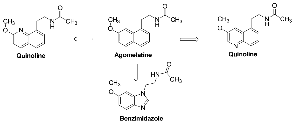
Figure 1. Aza-agomelatine derivatives
