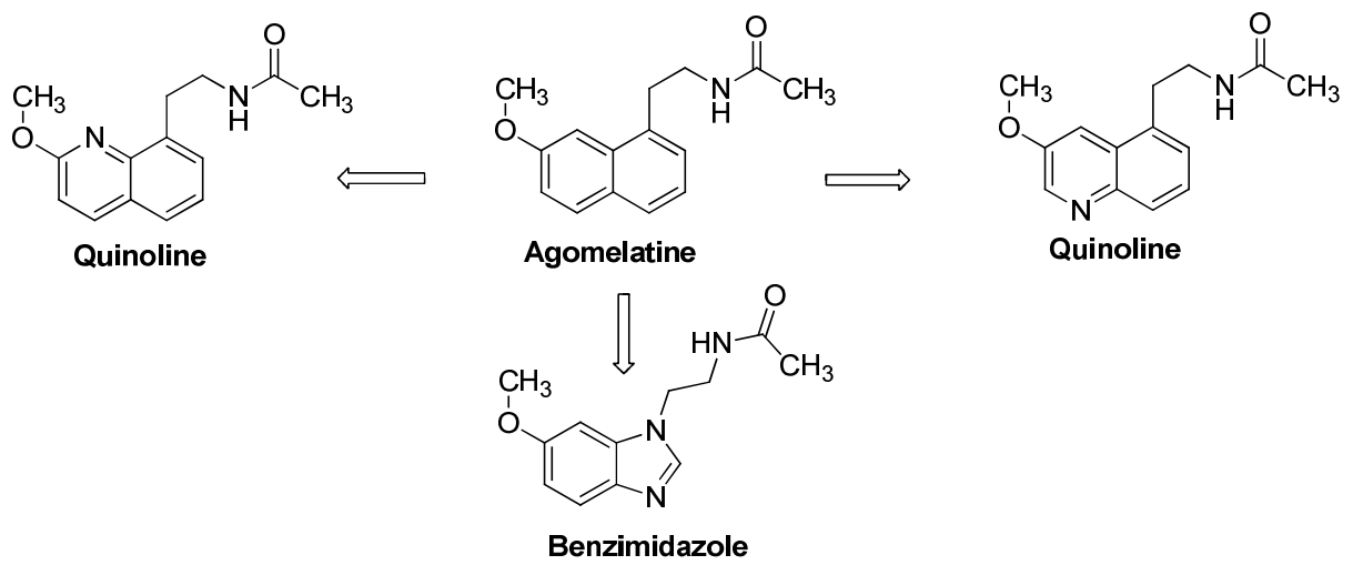
Figure 1. Aza-agomelatine derivatives
