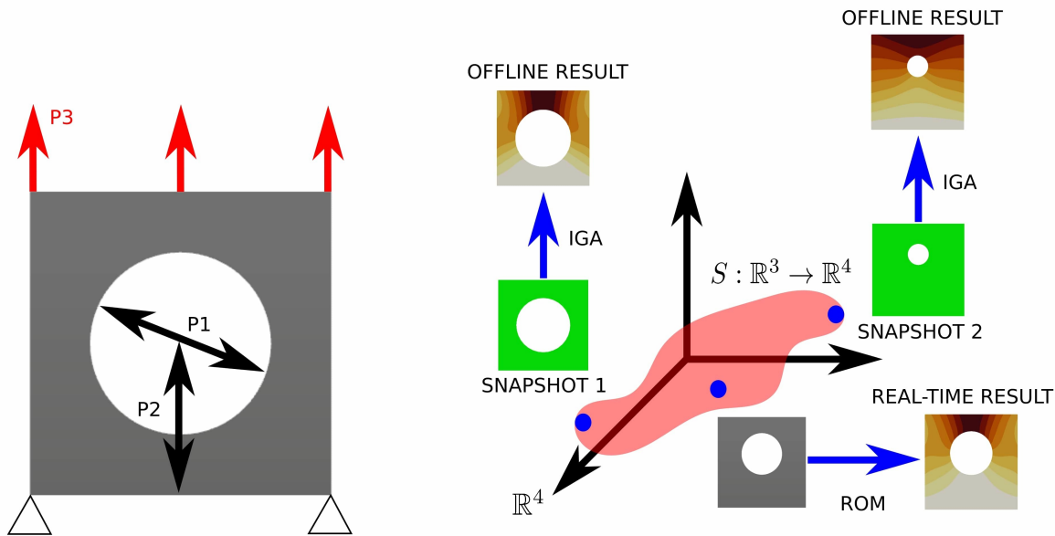
Figure 9: Reduced order model building and evaluation for a plate with one hole. Snapshots are calculated using IGA (IsoGeometric Analysis). P1 and P2 are geometrical parameters defining respectively the diameter and the position of the hole along his height. P3 is a loading parameter. Response surfaces S are embedded in 4-dimensional space. There are as many surfaces as there are modes in the reduced basis.
