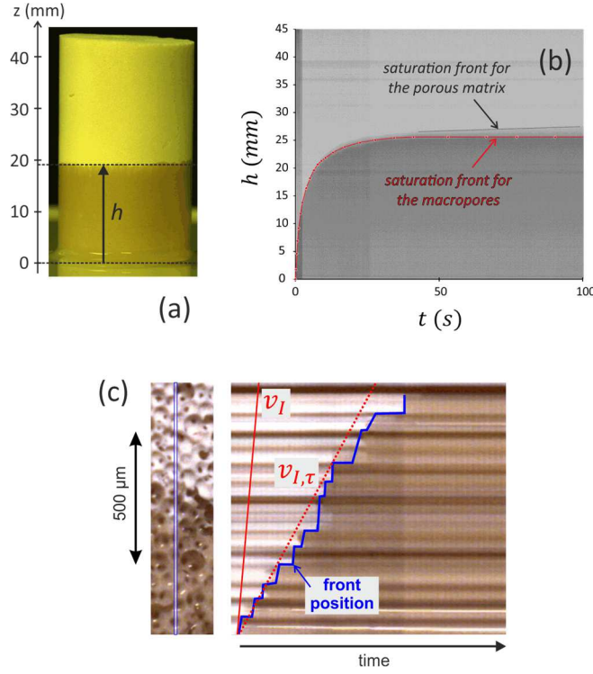
Figure 3: Imbibition experiment. (a) Image of the solid foam sample during imbibition. The sample is put in contact with water solution and the wet front height, h , is followed as a function of time. The front rise is better highlighted through the space-time image shown in (b). The red points and line highlight the water saturation front for the foam pores (macropores). The dotted line highlights the water saturation front in the porous solid skeleton of the foam. The corresponding velocity is small, so the second front is better distinguished after the water front stops in the macropores. (c) Close-up of the pore filling process during imbibition (left) and corresponding space-time image (right). The blue line shows the positions of the water front.
