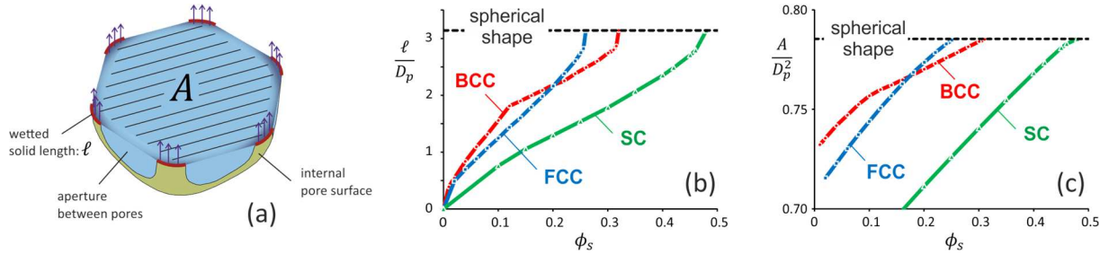
Fig. 6: (a) Sketch of single representative foam pore (cut at the middle cross-section for clarity). In each pore, surface tension acting at the solid surface (shown by the arrows) supports the column of liquid beneath the interface. (b) Wetted solid length \ell divided by D_p as a function of solid volume fraction for three ideal foam structures: FCC, BCC (Kelvin) and SC. (c) Pore cross section A divided by D_p^2 for three ideal foam structures: FCC, BCC (Kelvin) and SC.
