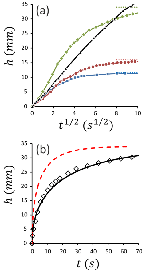
Figure 4: Typical imbibition curves, i.e. capillary rise height as a function of time. (a) Height h as a function of t^{1/2} for samples. Squares: D_p = 1030 \mu\text{m} and \phi_s = 0.33 ; Circles: D_p = 630 \mu\text{m} and \phi_s = 0.28 ; Diamonds: D_p = 300 \mu\text{m} and \phi_s = 0.17 ; Triangles: D_p = 195 \mu\text{m} and \phi_s = 0.18 . The dotted lines corresponds observed saturation heights. (b) Height h as a function of time for sample characterized by D_p = 300 \mu\text{m} and \phi_s = 0.17 . Solid line corresponds to equation 2 with parameters: \Delta P_c = 333 \text{ Pa} (equivalently h_\infty = 34 \text{ mm} ), k_I = 6 \cdot 10^{-11} \text{ m}^2 . The dashed line corresponds to equation 2 with parameters: \Delta P_c = 333 \text{ Pa} (equivalently h_\infty = 34 \text{ mm} ), k_I = k_D = 22.6 \cdot 10^{-11} \text{ m}^2 .
