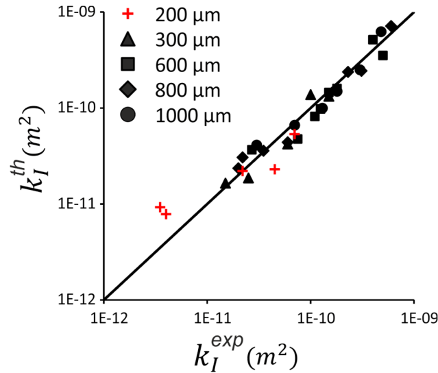
Figure 8: Permeability values given by eq. 7 as a function of permeability values deduced from imbibition experiments. In eq. 8, k_D values are given by eq. 5, \Delta P_c values are presented in Fig. 5a, and f = \alpha(D_p/\kappa^{-1})\phi_s^{3/2} with \alpha = 34 \cdot 10^3 . Each symbol corresponds to a given pore size, as indicated.
