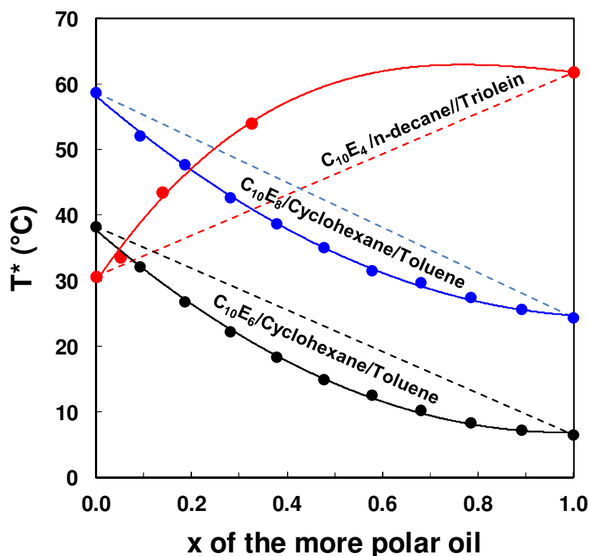
Figure 11. Fish-tail-temperatures of mixtures of cyclohexane and toluene at different molar fractions of the more polar oil using either (●) C_{10}E_8 or (●) C_{10}E_6 as surfactants [103]. Fish-tail-temperatures of mixtures of triolein and n-decane at different molar fractions using (●) C_{10}E_4 as surfactant [32]. The dotted line indicates the hypothetical linear behaviour of fish tail temperature as a function of oil composition.
