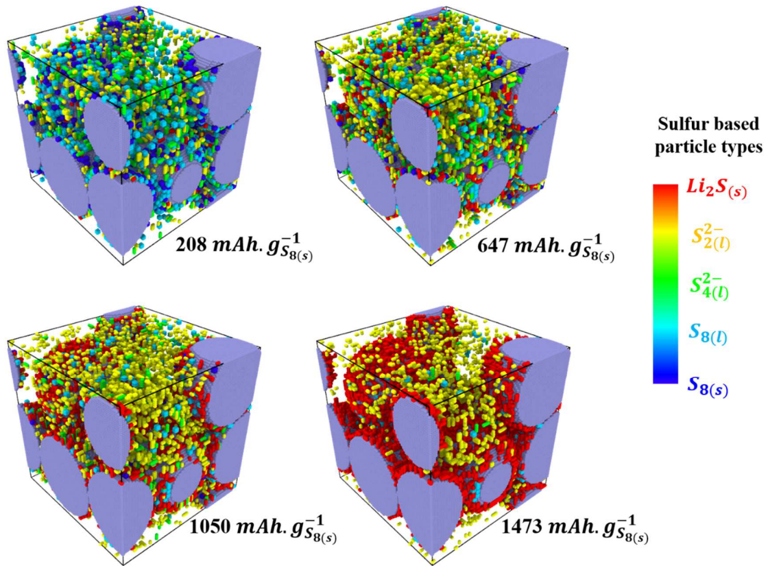
Figure 4. Visualization of the simulation box at 208, 647, 1050 and 1473 mAh.g_{S_{8(s)}}^{-1} during the 2C discharge simulation. The colour map in the image shows the colour coding assigned to different types of sulfur based particle types, where S_{8(s)} , S_{8(l)} , S_{4(l)}^{2-} , S_{2(l)}^{2-} and Li_2S(s) particles are shown in navy blue, sky blue, green, yellow and red respectively.
