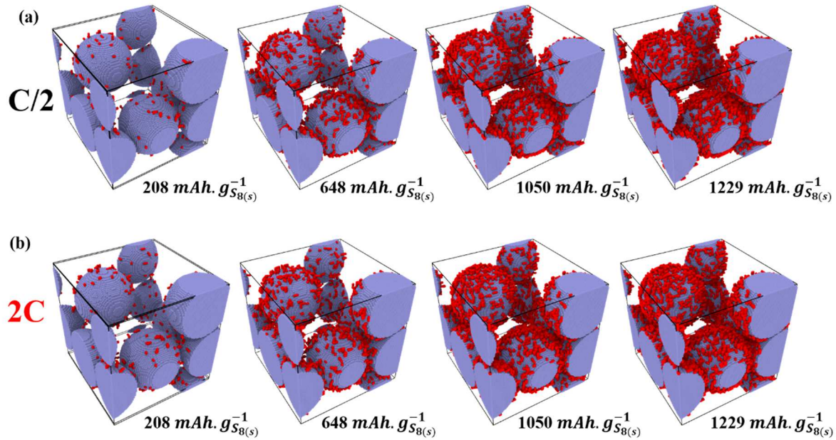
Figure 8. Visualizations of Li_2S_{(s)} deposits (in red) over the surface of the carbon particles at 208, 648, 1050 and 1229 mAh \cdot g_{S_8(s)}^{-1} during (a) C/2 and (b) 2C discharge simulations.
