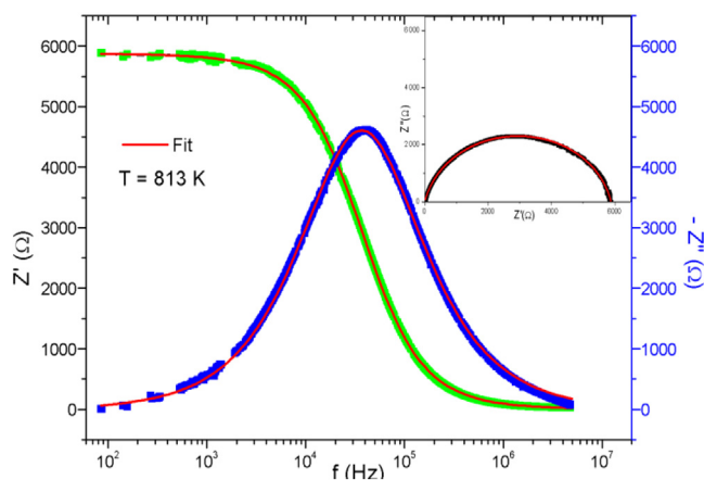
Figure 8 Variation of real and imaginary parts of impedance with frequency. Inset: Nyquist plots ( -Z'' vs. Z' ) of impedance data at temperature T = 813 K for \text{La}_{1.85}\text{Ca}_{0.15}\text{CuO}_{3.5} compound.
