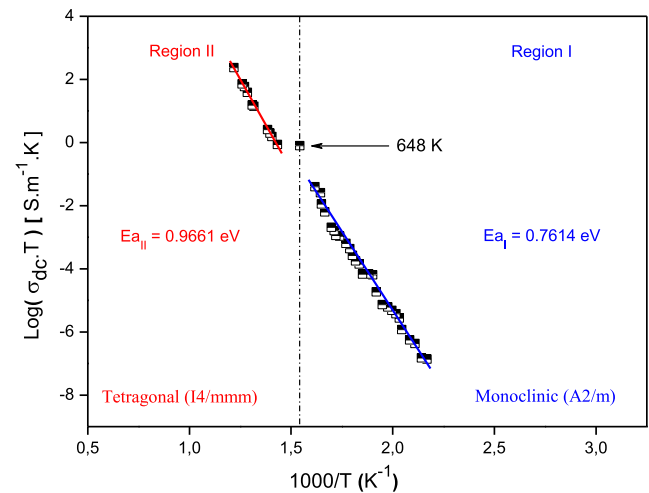
Figure 10 Arrhenius relation of \text{Log}(\sigma_{dc}T) with the reciprocal of absolute temperature ( 10^3/T ) for the \text{La}_{1.85}\text{Ca}_{0.15}\text{CuO}_{3.5} compound.
