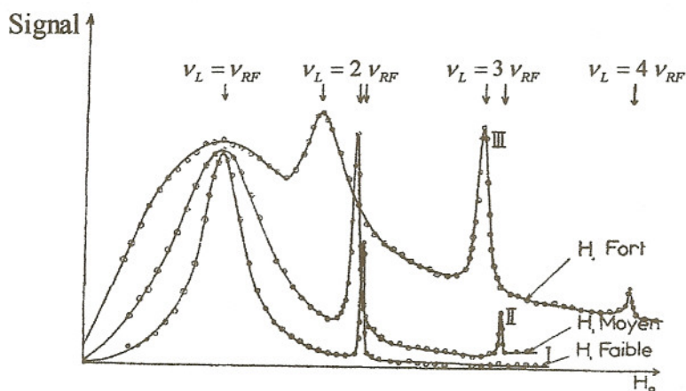
Fig. 7. Spectrum of multiphoton RF resonances m_F \rightarrow m_F + 1 observed in the ground state of optically pumped sodium atoms. The curves I, II, III correspond to increasing powers of the RF field (Figure taken from Ref.[9]).
