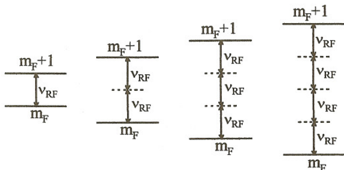
Fig. 6. Multiphoton RF resonances between 2 Zeeman sublevels m_F and m_F+1 . For a n -photon resonance, the frequency \nu_{RF} of the RF field is a subharmonic \nu_L/n of the Larmor frequency \nu_L which determines the splitting between the 2 Zeeman sublevels.
