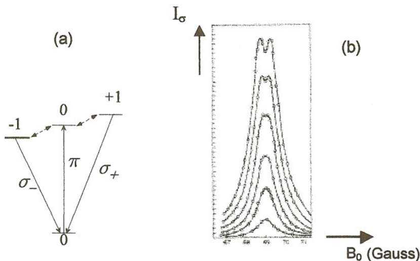
Fig. 1. (a) : Zeeman components of a transition 0 \leftrightarrow 1 . The excitation is \pi -polarized and one observes the \sigma -polarized reemitted light. (b) : Variations of the \sigma -polarized reemitted light versus the magnetic field which splits the 3 excited Zeeman sublevels. The various curves correspond to different values of the amplitude of the RF field which induces resonant transitions between the excited Zeeman sublevels. The amplitude of the RF field increases by a factor 7 between the smallest curve and the largest one.
