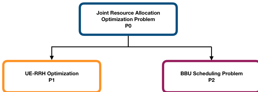
Figure 4: The two-stage resource allocation problem
