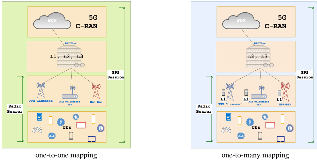
Figure 2: One-to-one vs One-to-many BBU-RRH mapping
