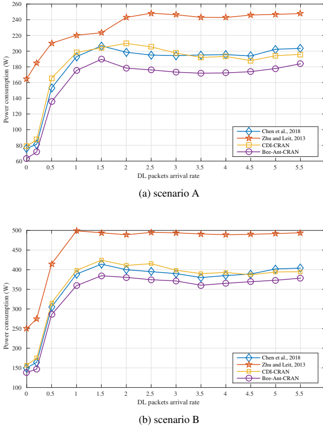
Figure 7: Power consumption
