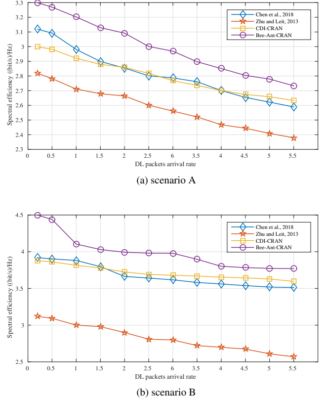
Figure 8: Spectral efficiency
