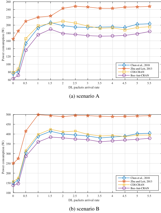
Figure 7: Power consumption
