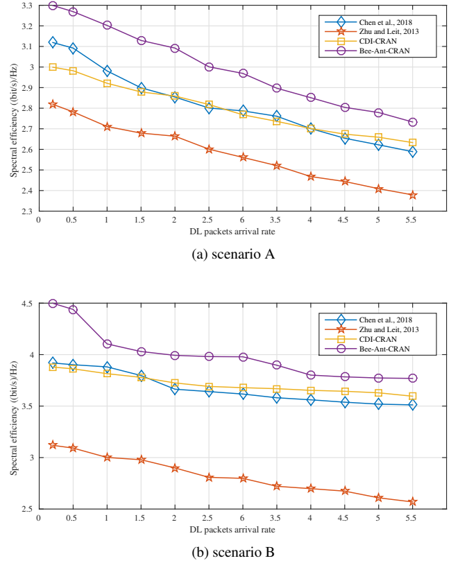
Figure 8: Spectral efficiency
