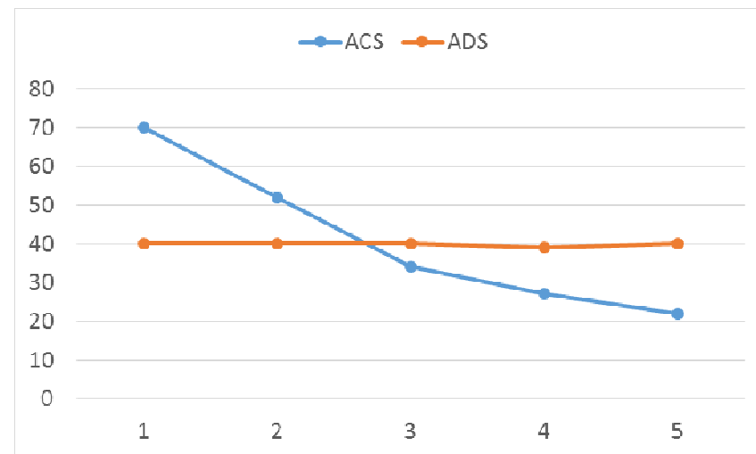
b) Number of optimal solutions for different values of |K|
