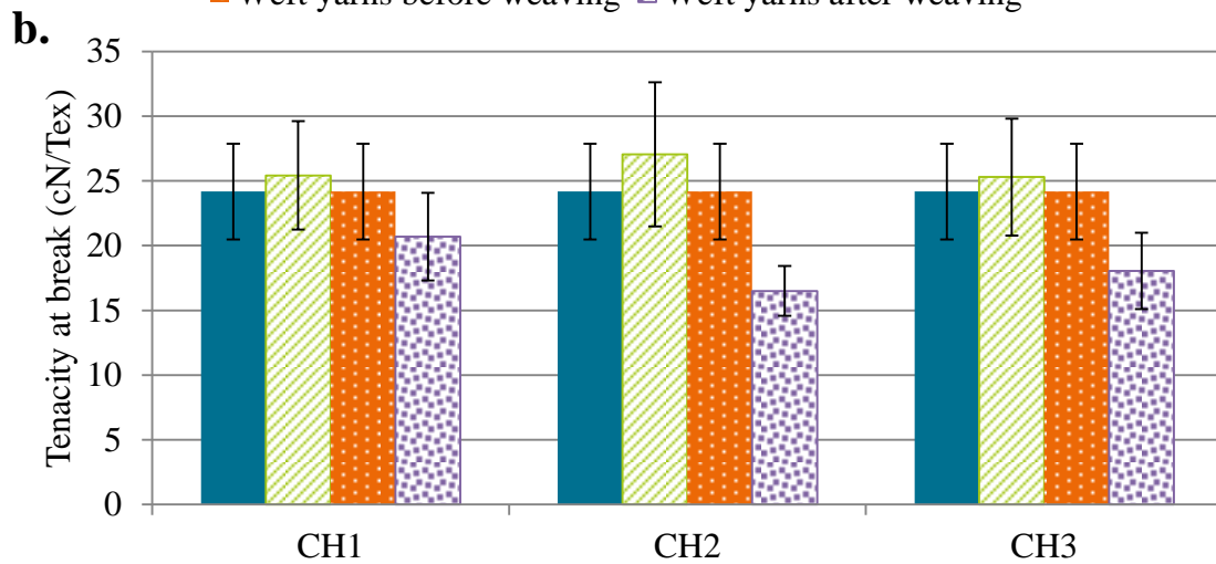
Figure 6 : Influence of weaving process on yarns properties a. Twist level b. Tenacity at break
