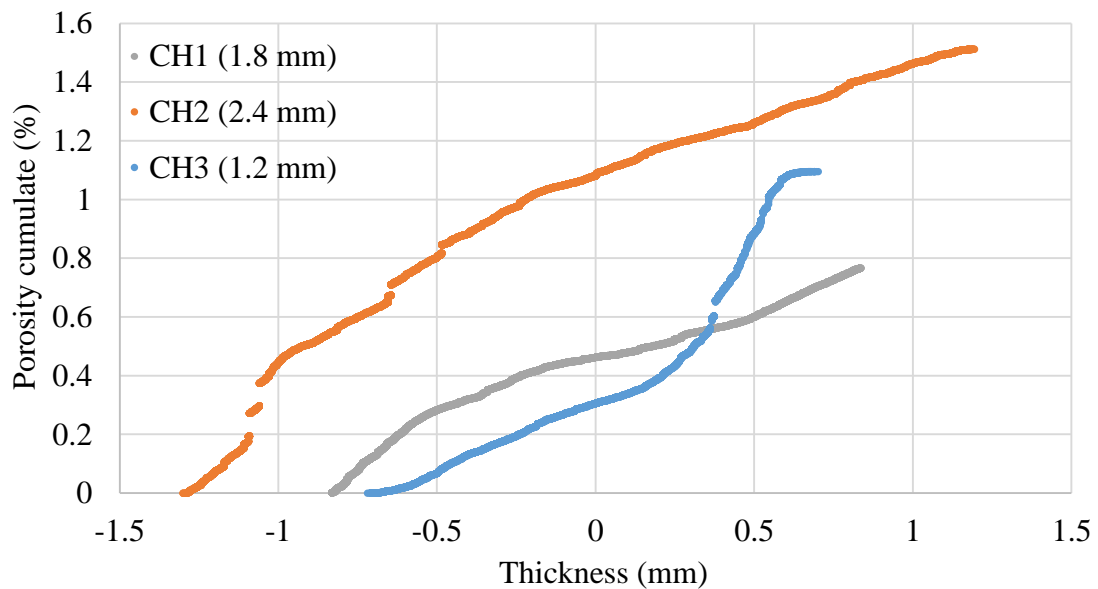
Figure 12: Distribution of porosities through the thickness of the composite samples
