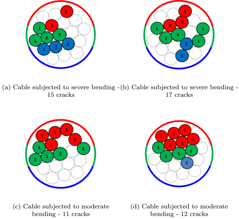
Figure 10: Projections of the fatigue cracks in a transverse cut of the cable. The red color indicates points above the median fiber (top of the bent cable); the blue color indicates the points below the median fiber (bottom of the bent cable); the green color the points at the level of the median fiber.
