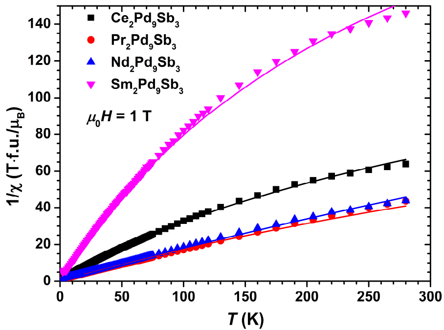
Fig. 11. Reciprocal susceptibility vs temperature for \text{Ln}_2\text{Pd}_9\text{Sb}_3 ( \text{Ln} = \text{Ce}, \text{Pr}, \text{Nd}, \text{Sm} ) samples in a magnetic field \mu_0 H = 1 \text{ T} (solid lines – modified Curie-Weiss fit)
