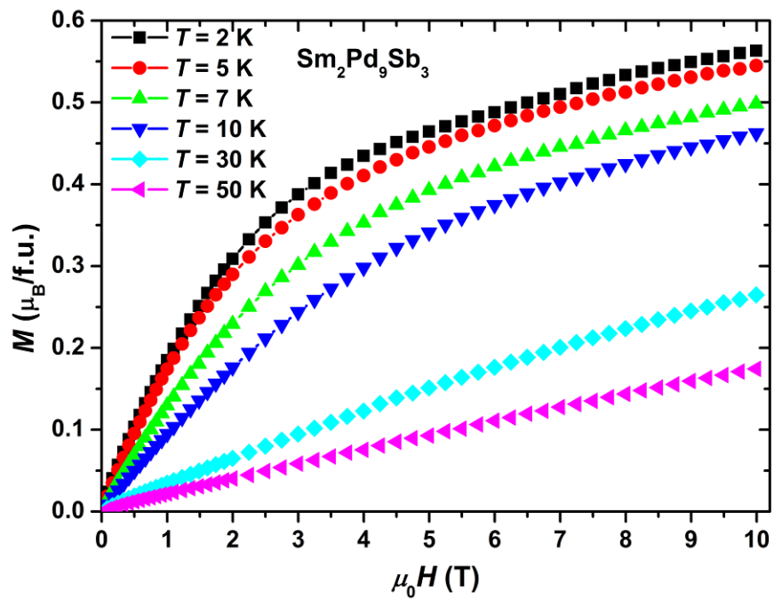
Fig. 7. Isothermal magnetization curves of \text{Sm}_2\text{Pd}_9\text{Sb}_3 recorded at the indicated temperature.
