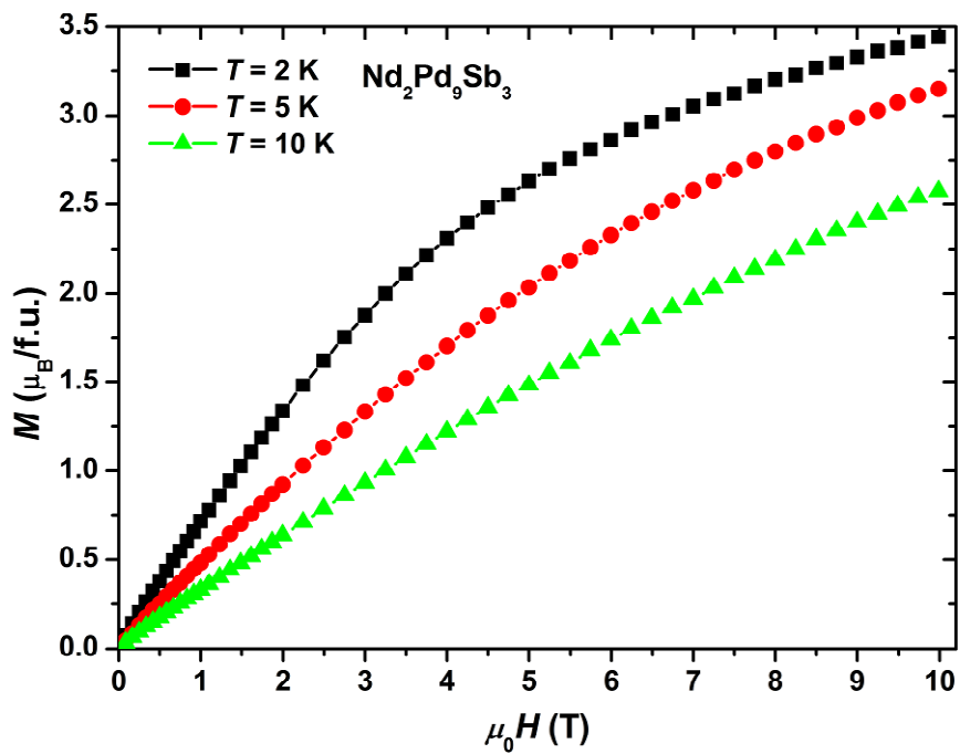
Fig. 9. Isothermal magnetization curves of \text{Nd}_2\text{Pd}_9\text{Sb}_3 recorded at the indicated temperature.
