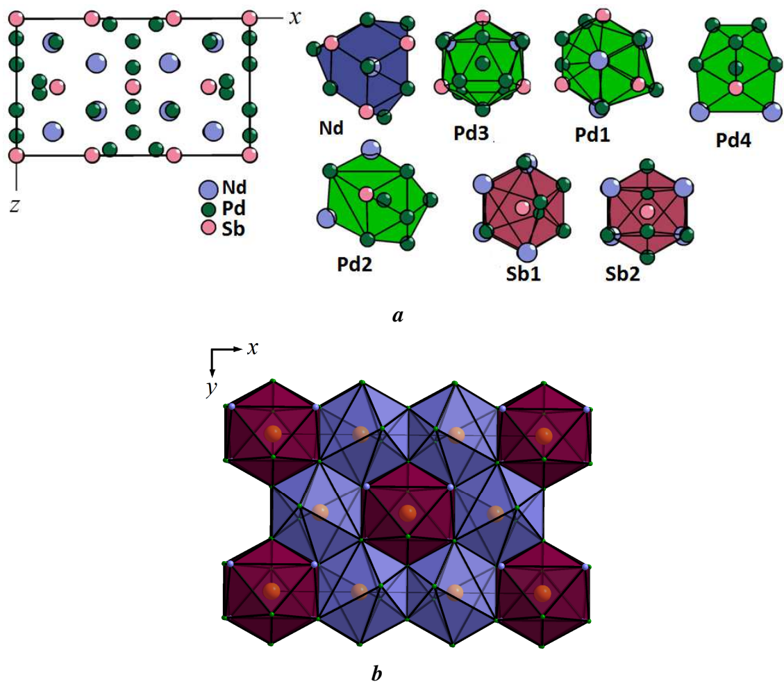
Fig. 2. (a) – Crystal structure of the \text{Nd}_2\text{Pd}_9\text{Sb}_3 antimonide ( \text{Ce}_2\text{Pd}_9\text{Sb}_3 type), coordination polyhedra of atoms; (b) – arrangement of Sb1 (blue) and Sb2 (red) polyhedra in the structure, the size of the atoms Pd and Nd is reduced for better perception.
