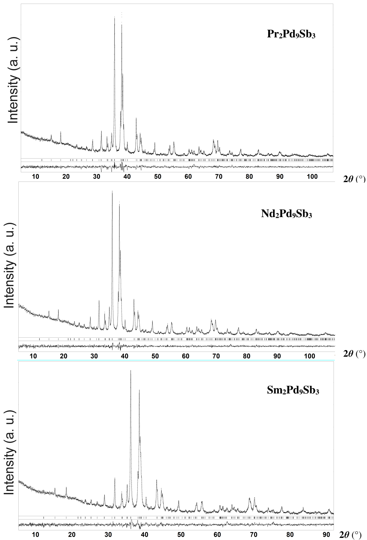
Fig. 1. Observed (dots), calculated (line) and difference (bottom line) XRD profiles for Ln_2\text{Pd}_9\text{Sb}_3 samples ( Ln = \text{Pr}, \text{Nd}, \text{Sm} ).
