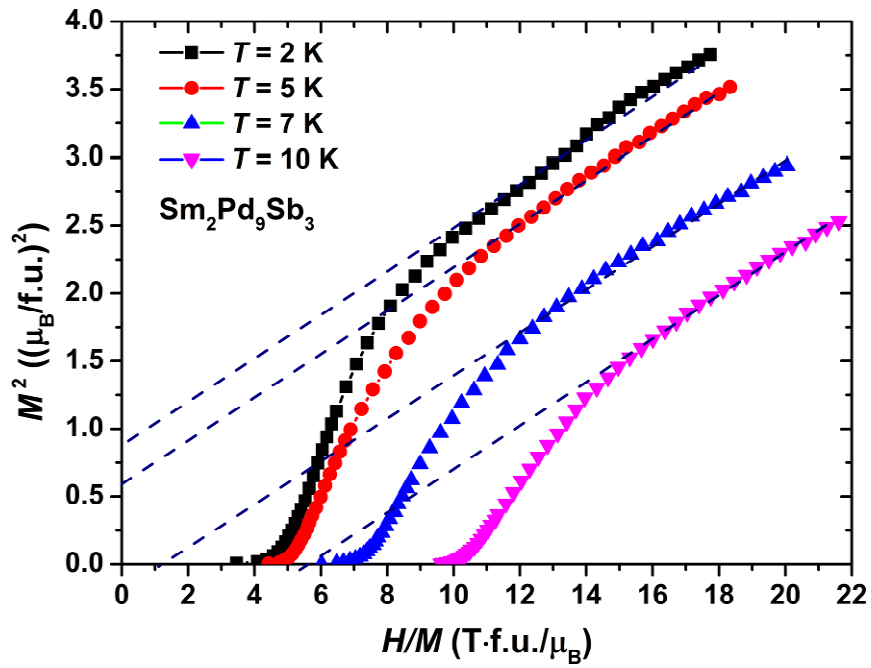
Fig. 6. Arrott-Belov plots for \text{Sm}_2\text{Pd}_9\text{Sb}_3 , at the indicated temperature.
