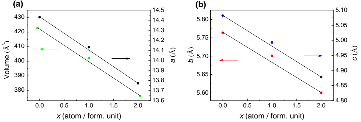
Figure 2: Room temperature unit-cell parameters comparison for \text{MnNb}_{2-x}\text{V}_x\text{O}_6 columbites ( x = 0, 1 and 2 ).
