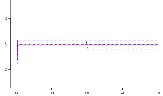
Estimation of \sigma^2 + \xi^2
