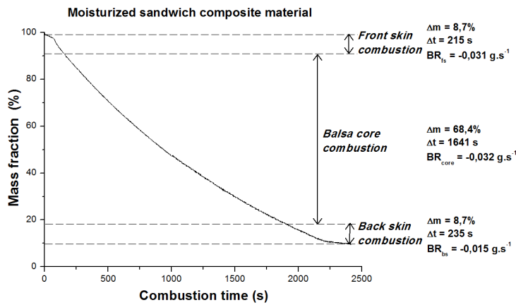
Figure 9. Wet sandwich sample: kinetics of combustion of the sandwich composite material.
