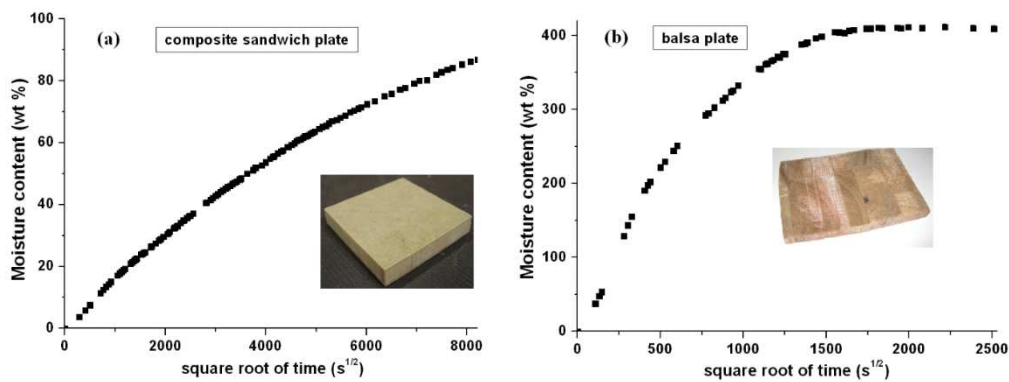
Figure 4. Kinetics of water diffusion at 40°C, in (a) a plate of sandwich composite material and in (b) a plate of balsa (alone without skins) infused with resin (plates size: 128 x 126 x 18a or 15b mm 3 ).
