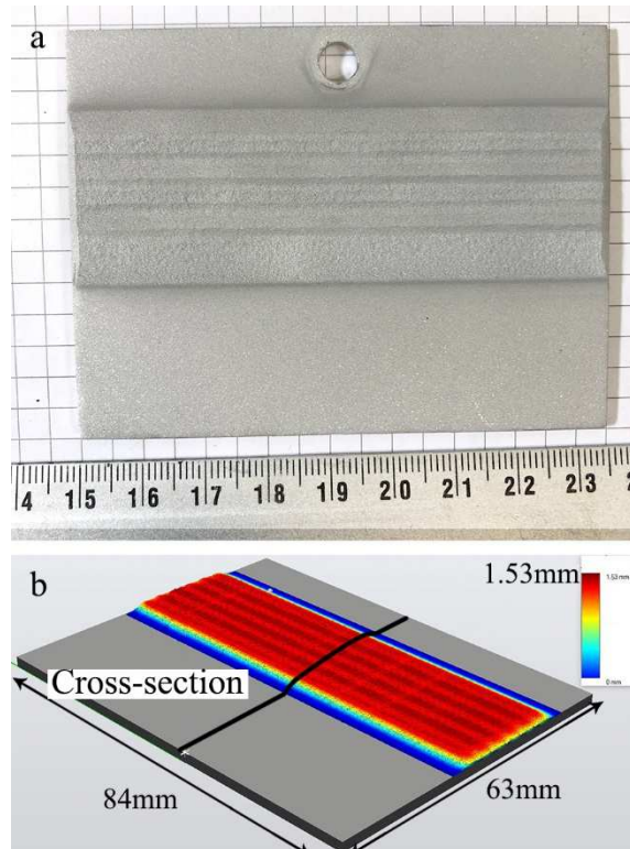
Fig-14. Fig. 15. (a) Experimental result; (b) Simulation result.
