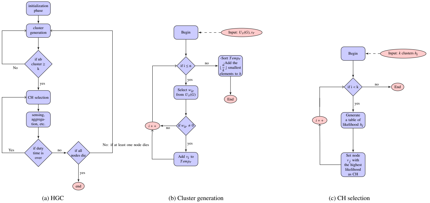
Figure 4: Flowcharts
