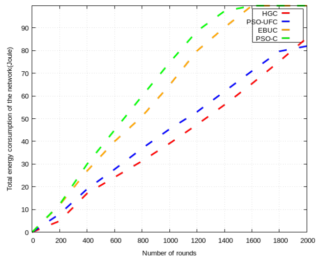
(a) Energy consumption of the network: WSN#1
