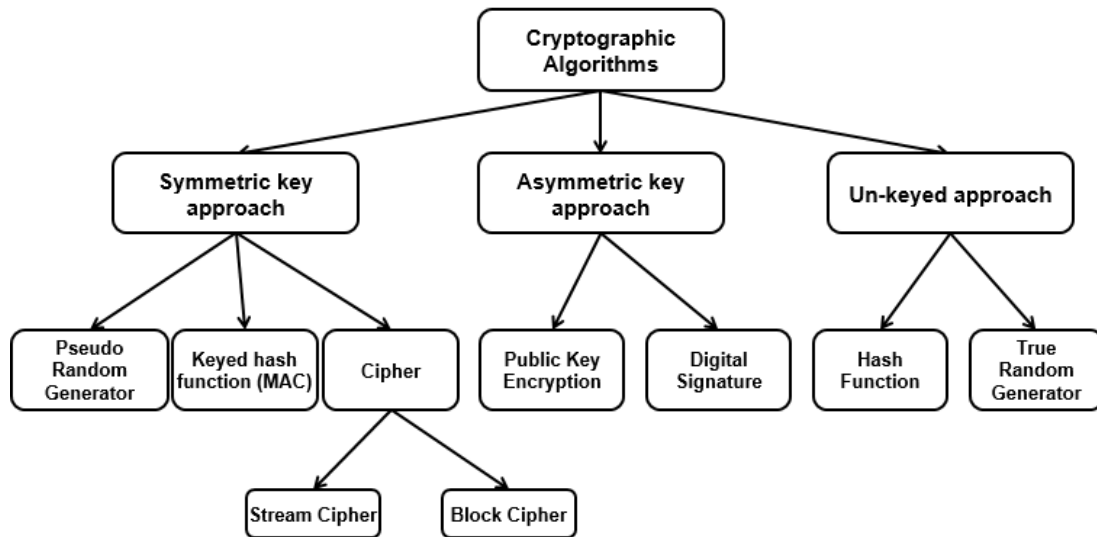
Fig. 12: Existing Cryptographic Algorithms
