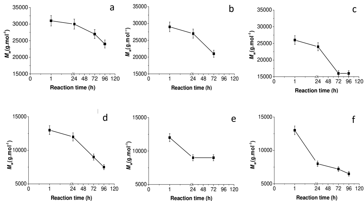
1 2 Fig. 5. Effect of enzyme concentration on M_w of P and S as a function of reaction time with the 3 enzyme/polymer ratio of 30\mu\text{L.g}^{-1} (a, d); 50\mu\text{L.g}^{-1} (b, e) and 180\mu\text{L.g}^{-1} (c, f).
