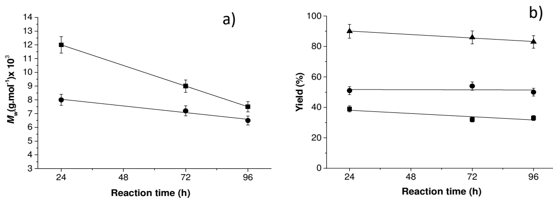
5 6 7 Fig. 6. a) Weight average molar mass decrease of S fractions using (■) 30 and (●) 180\mu\text{L.g}^{-1} 8 enzyme/polymer ratio as a function of reaction time. b) Yield of depolymerized HMPC fraction 9 P (■), S (●) and total yield (▲) as a function of reaction time using 180\mu\text{L.g}^{-1} enzyme/polymer 10 ratio.
