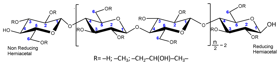
20 Fig. 1. Molecular structure of hydroxypropylmethyl cellulose (HPMC).
