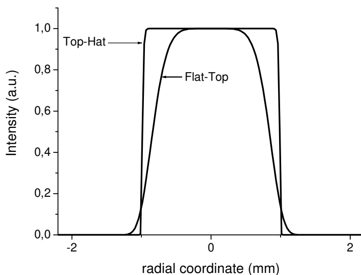
Figure 1: Flat-Top and Top-Hat intensity profiles.
