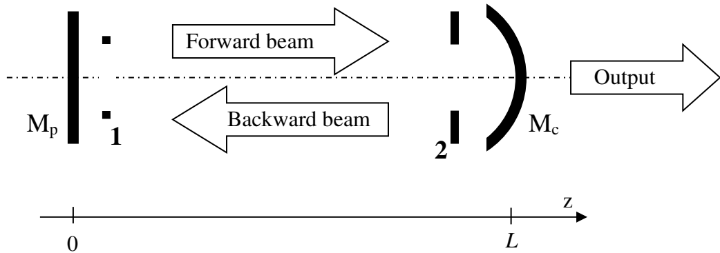
Figure 3: Scheme of the laser cavity of length L made up of a plane mirror M_p and a concave mirror M_c of radius of curvature noted R . The transverse mode selection is achieved by the combined effects of a circular aperture (2) against M_c and a circular absorbing ring (1) set on M_p .
