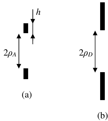
Figure 4: Geometry of (a): absorbing ring, and (b): circular aperture
