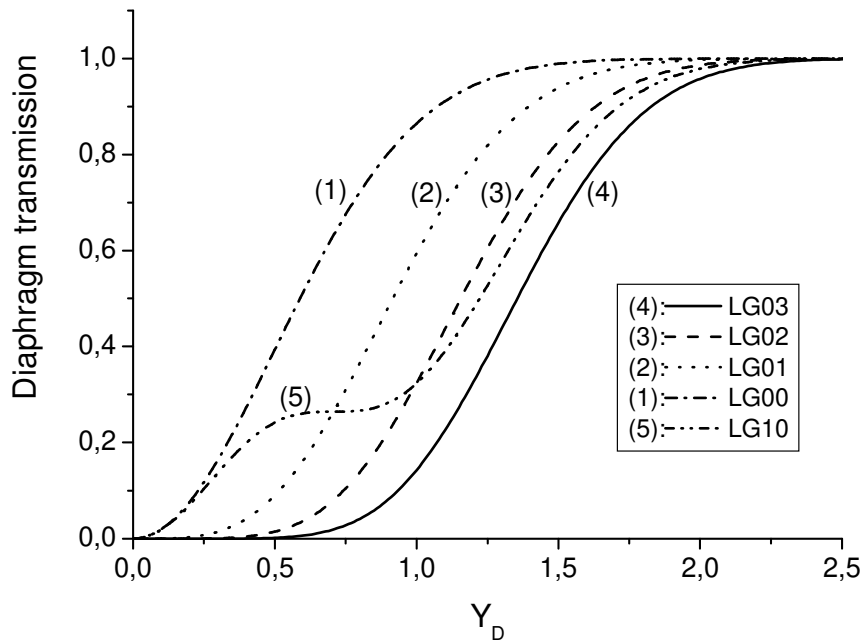
Figure 5: Variations of the single pass transmission for several LG_{pl} beams through a diaphragm of normalised radius Y_D .
