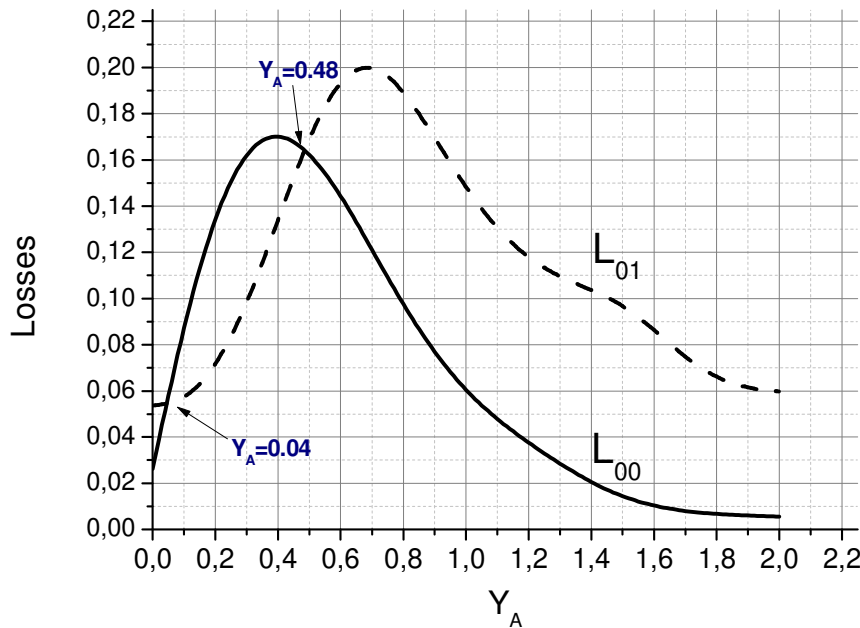
Figure 7: Variations of losses L_{00} and L_{01} versus parameter Y_A for L=252\text{mm} , g=0.5 , Y_D = 1.6 , h=20\mu\text{m} . W_p = 292\mu\text{m} , W_c = 649\mu\text{m} .
