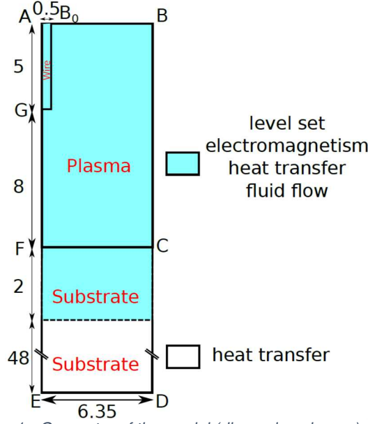
Fig. 1 - Geometry of the model (dimensions in mm)
