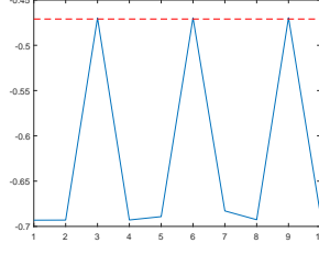
Figure 1: Plot of L_{n,d}/n (solid line) and \mathcal{L}_3 (dashed line), for d \in \{1, \dots, 10\} .
