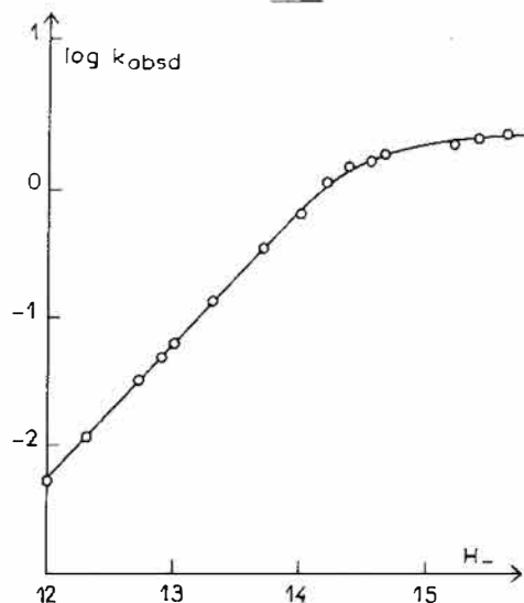
Figure 1. Plot of the logarithms of the observed rate constants k_{obsd} vs. H_- for the hydrolysis of p\text{-NO}_2\text{C}_6\text{H}_4\text{CH:NOCONHCH}_3 at 25^\circ\text{C} ( \mu 1.0, KCl, when [\text{OH}^-] < 1.0 \text{ N} ).
