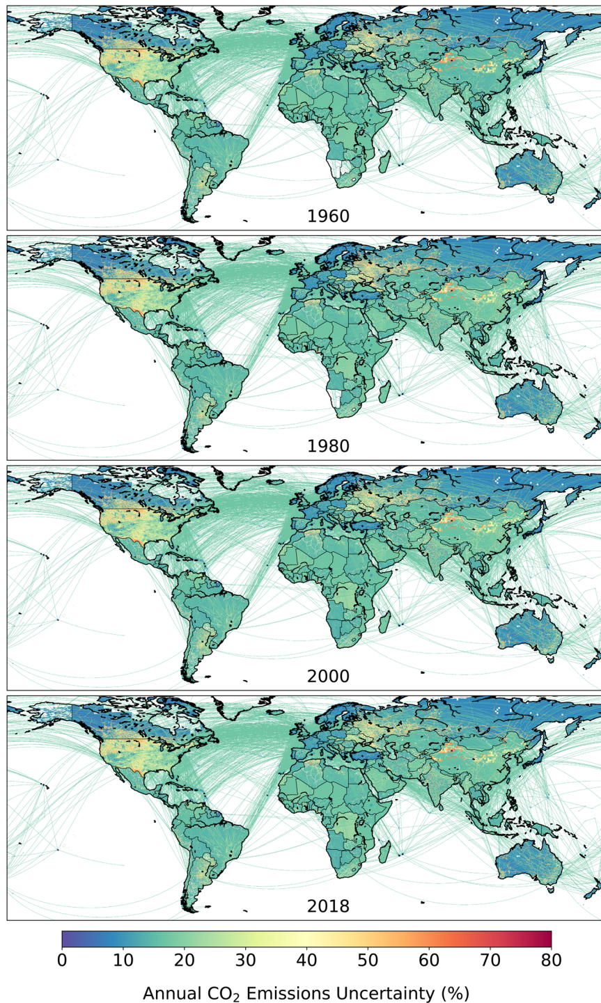
Fig. 11 Gridded ( 0.1^\circ \times 0.1^\circ ) estimates of relative uncertainty in total \text{CO}_2 emissions for four years of the GCP-GridFEDv2019.1 time series. Uncertainty in total emissions is aggregated from the sector-level estimates (see Table 2). The uncertainty estimates account for uncertainty across national emission reports and spatial differences in the sectoral breakdown to total emissions in each grid cell, which changes throughout the time series, however they exclude uncertainties associated with the spatial or temporal (monthly) disaggregation of national emissions (see ‘ \text{CO}_2 emissions uncertainty’). Aggregation of uncertainties to a coarser resolution should account for the non-independence of gridded emissions uncertainties.
