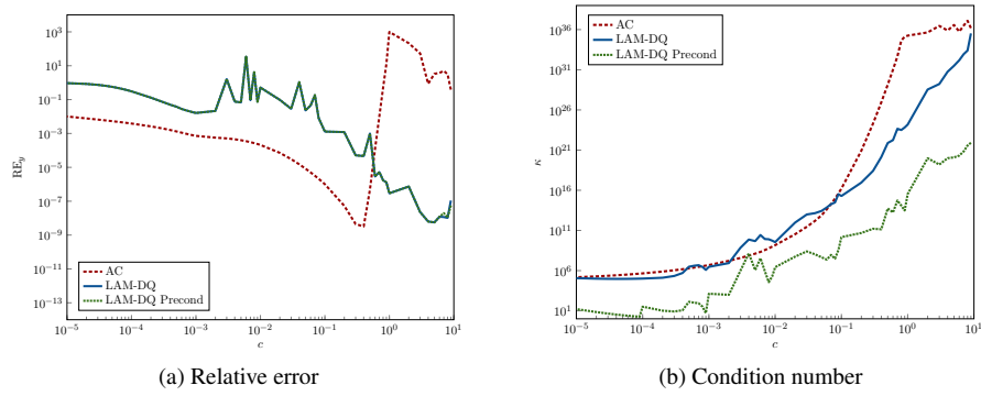
Figure 2: Comparison of different methods for \beta = 10^{-6}
