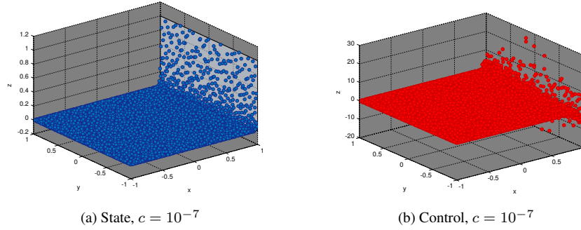
Figure 3: Solution for problem 2, n = 50000 , \beta = 10^{-6}
