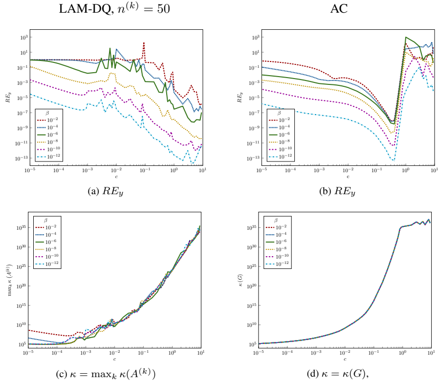
Figure 1: Comparison between the values of the relative error ( RE_y ) and the condition number ( \kappa ), by varying the shape parameter c . These calculations were obtained using quadruple precision, and different values of the penalty constant \beta .
