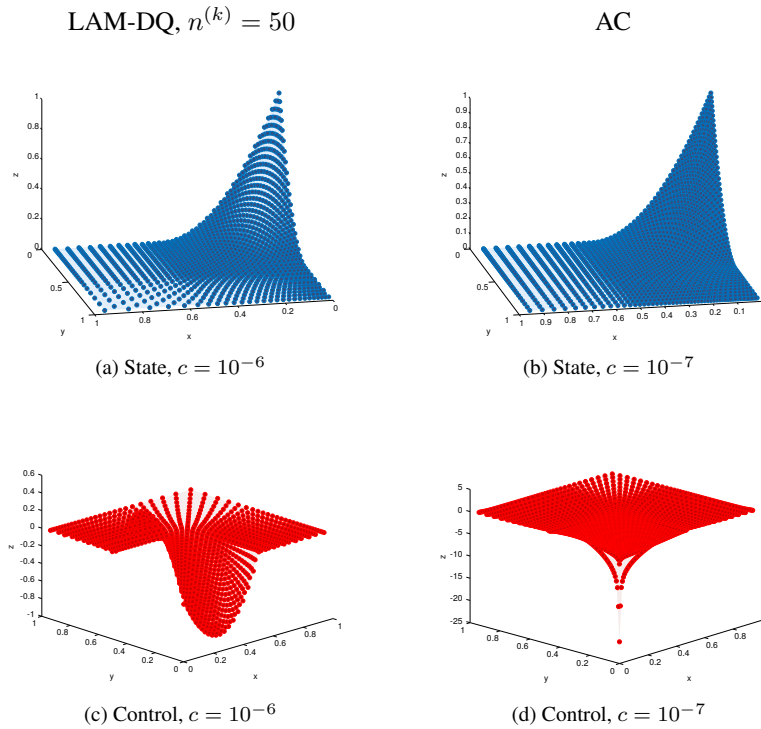
Figure 4: Solution for problem 3, n = 3021 , \beta = 10^{-10}
