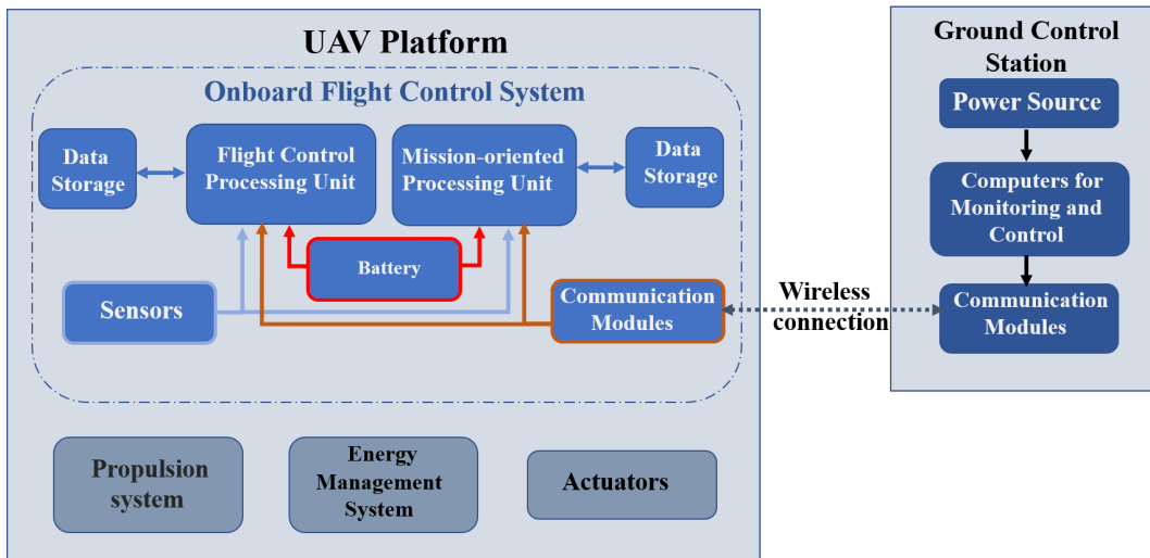
Figure 2: Block diagram of a typical UAS.
