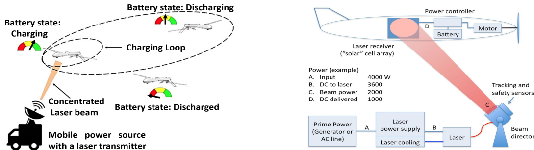
Figure 16: Laser-powered UAVs [110, 112].
