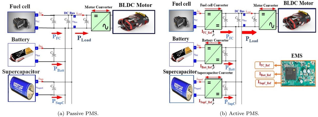
Figure 25: Active vs passive PMS Architectures.
