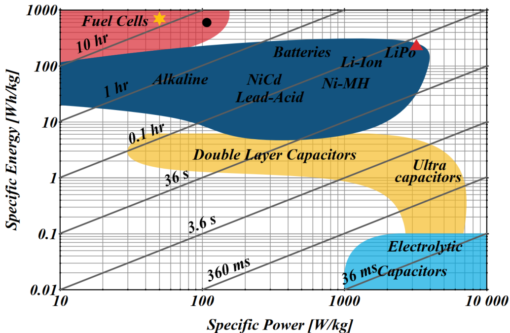
Figure 19: Specific energy/power comparison between energy sources [118].
