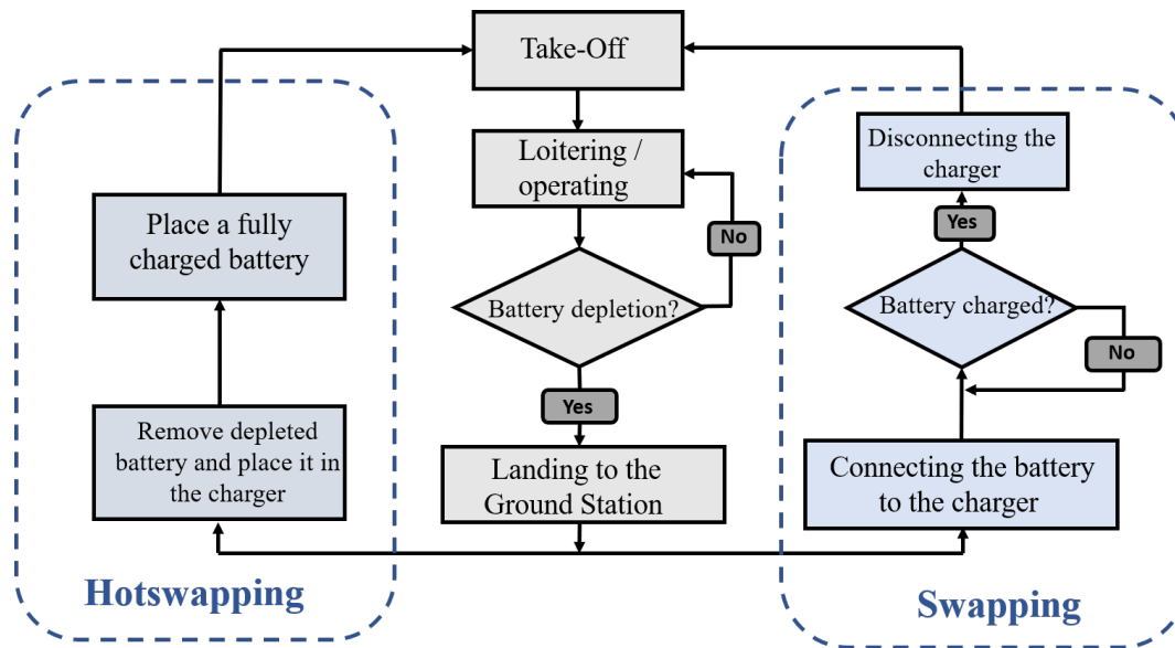
Figure 14: Swapping and Hotswapping Algorithms.
