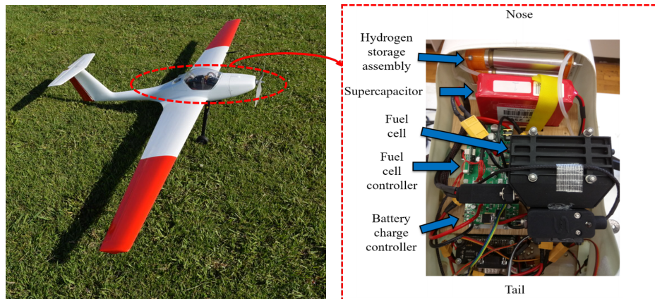
Figure 24: A hybrid fuel cell-battery-supercapacitor power supply in a UAV [17, 162].
