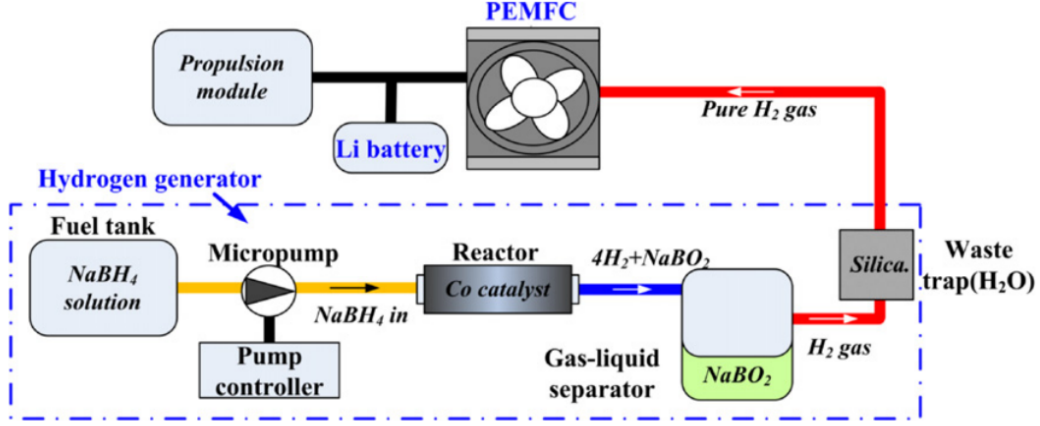
Figure 21: Fuel cell system auxiliaries illustration [123].
