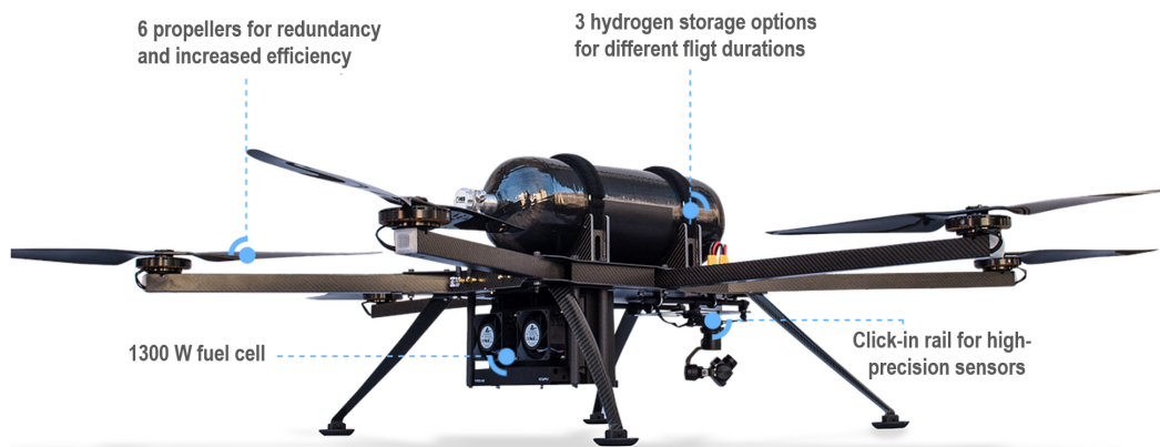
Figure 20: The Hycopter UAV from HES [121].
