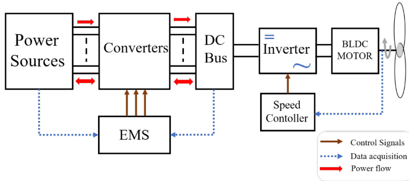
Figure 3: Block diagram of a UAV propulsion system.
