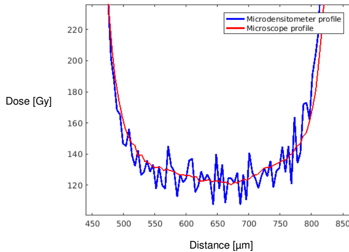
Figure 5. Valley dose distribution profile obtained with the microdensitometer (blue) and the microscope (red)
