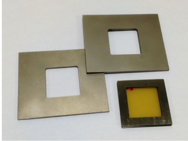
Figure 3. Metal masks used for the film readout. In the bottom right corner, one piece of radiochromic film is held between two metal masks.
