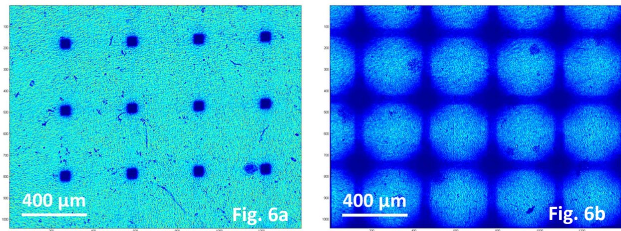
Figure 6a. Digital microscope image of pencil beams for peak dose evaluation. Figure 6b. Microscope image of pencil beams irradiated with 65000 Gy in the peak; the mean valley dose between pencil beam is 142 Gy.
