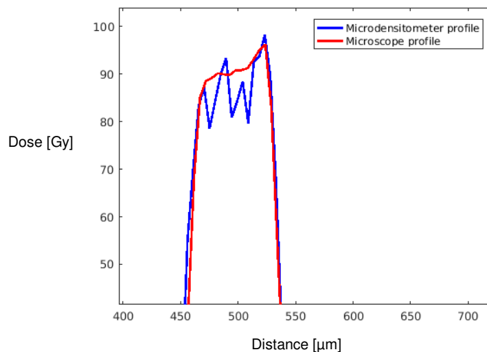
Figure 4. Peak dose profile of one single microbeam of 75 \mu\text{m} width (FWHM) obtained with the microdensitometer (blue) and the microscope (red)
