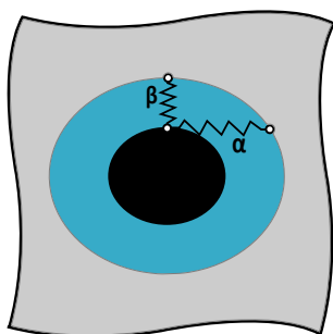
Figure 1: Imperfect interface modelled by a linear spring
