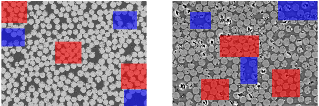
Figure 4: S.E.M. images of glass/polyester (left) and carbon/epoxy (right) microstructures.
