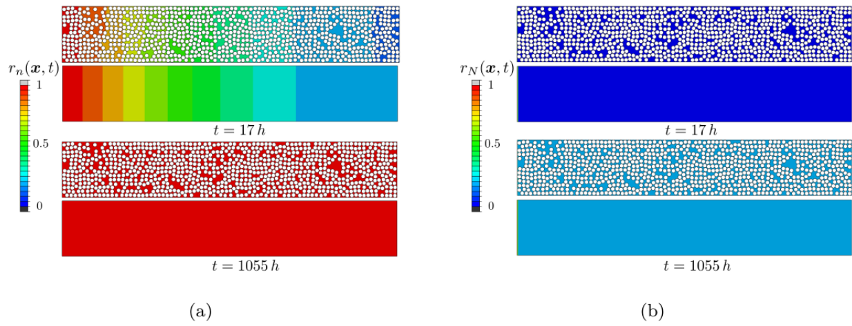
Figure 13: Free (a) and bounded (b) water molecules fields at two transient times t = 17h and t = 1055h for both heterogeneous and homogeneous cases.
