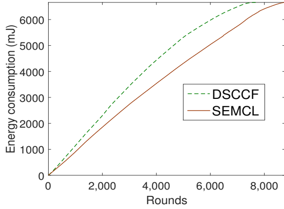
Figure 10: Network energy consumption per round
