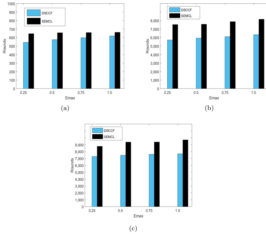
Figure 11: Node death varying with E_{max} (a) First Node Death (b) Half Node Death (c) Last Node Death
