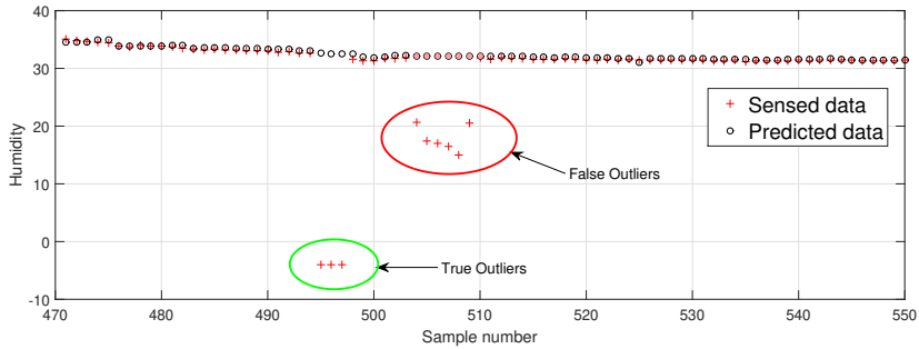
Figure 1: True outlier detection problem
