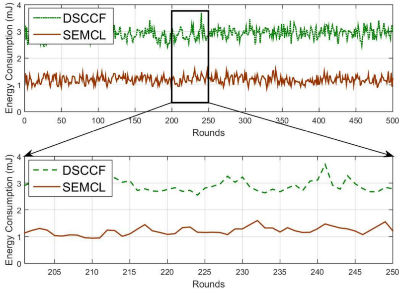
Figure 9: Energy consumption in clustering for whole network
