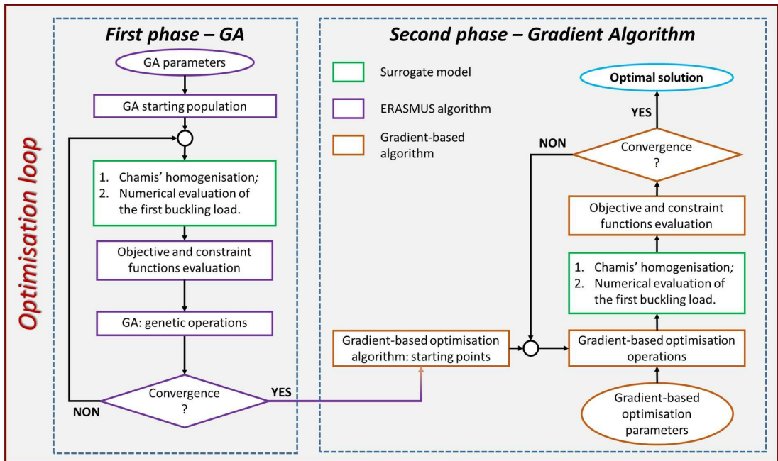
Figure 8: Optimisation strategy for the resolution of problem (21).
