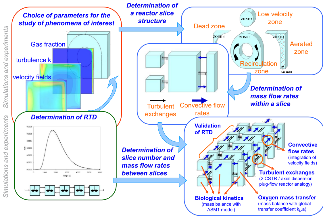
Figure 3: Construction procedure of Le Moullec (2010) compartmental model [58]
