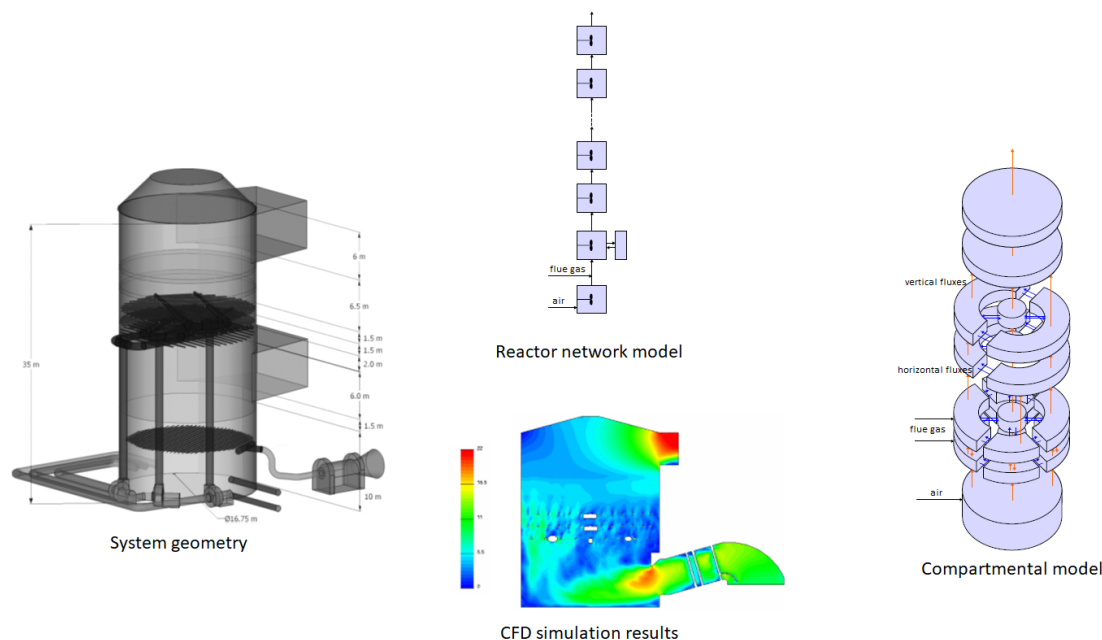
Figure 8: Examples of different modelling approaches applied to a Flue Gas Desulfurisation unit (adapted from [77])
