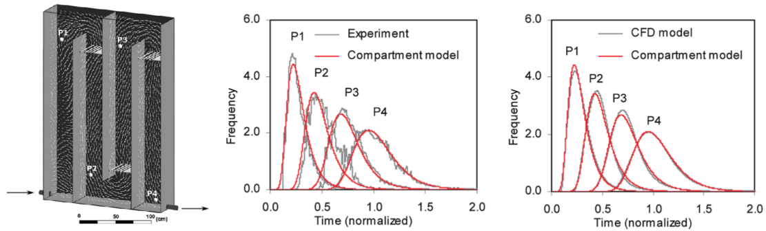
Figure 4: RTD curves at four sampling locations in the pilot reactor. These curves are normalised based on RTD curves at the outlet [34]
