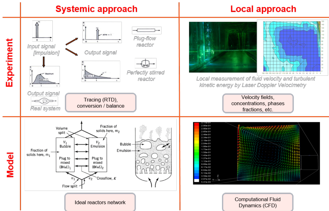
Figure 1: Comparison between systemic and local approaches (images adapted from Levenspiel [64] and Le Moulec [58])
