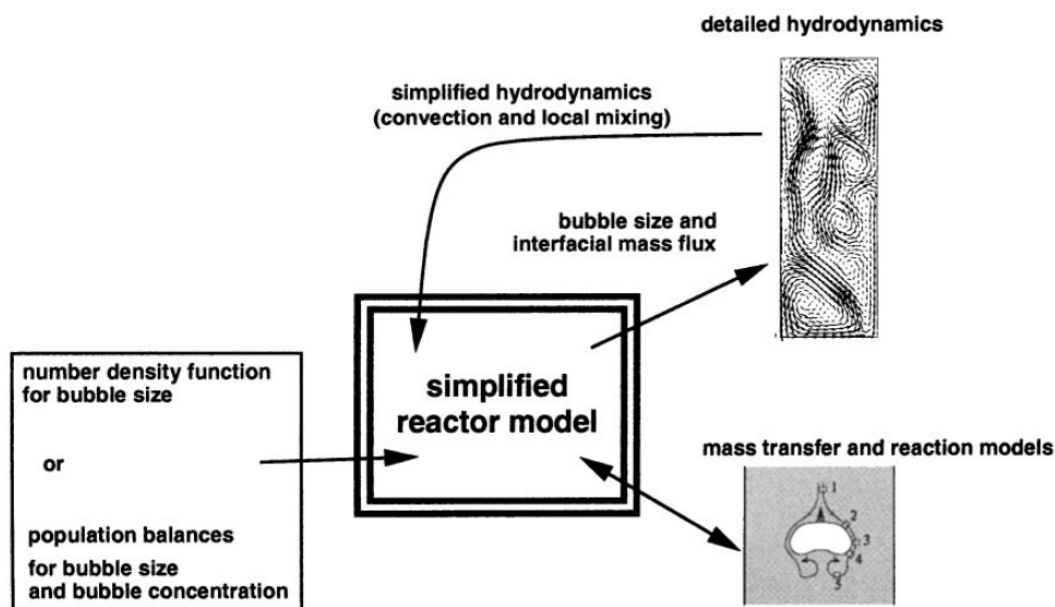
Figure 2: Multi-scale model of Bauer and Eigenberger [9]
