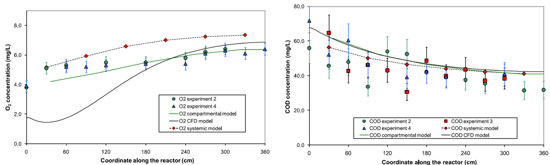
Figure 5: Comparison of Oxygen concentrations (left) and Chemical Oxygen Demand concentrations (right) for the three modelling approaches with experimental data [62]
