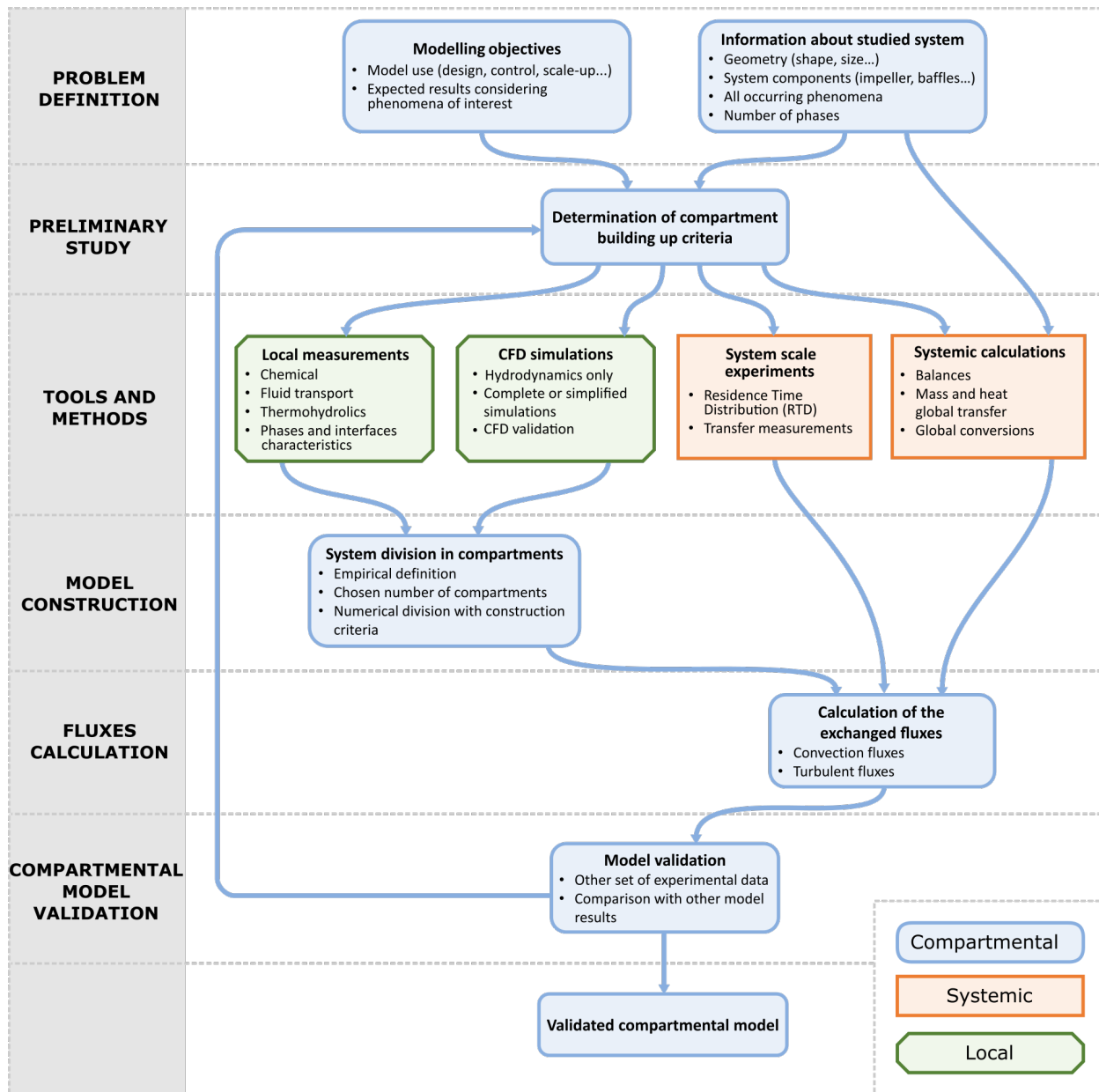
Figure 9: Proposed methodology for compartmental models construction
