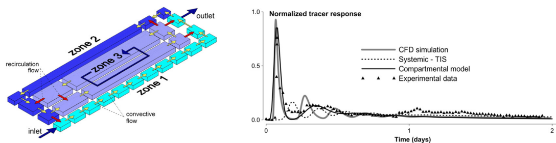
Figure 6: Representation of the compartmental model in the [5] study (left) and comparison of the RTD prediction with different models (right)
