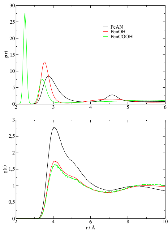
Figure 3: Upper panel: RDF of N \cdots O distance (PeAN) and O-H \cdots O (PenOH and PenCOOH). Lower Panel: correlations involving the terminal carbon atoms of the alkyl chains.
