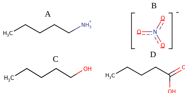
Figure 1: Sketch of the studied systems : (A) pentylammonium, (B) nitrate, (C) 1-pentanol and (D) 1-pentanoic acid.
