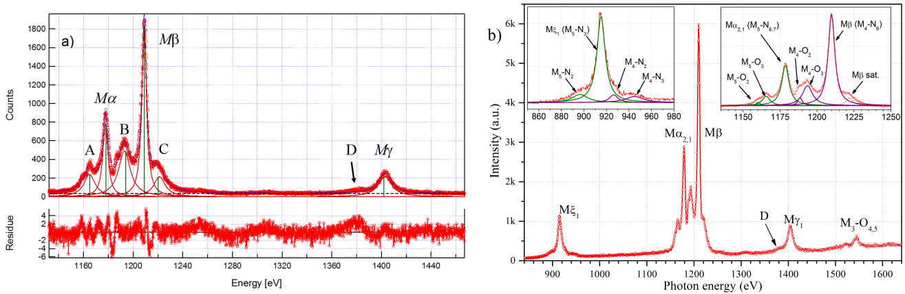
Figure 5: a) The observed M\alpha, \beta, \gamma spectrum of Gd obtained with the antiparallel double-crystal x-ray spectrometer with TAP(001) crystals in photon bombardment. Several peaks marked by A, B, C, and D are shown together with Lorentzian functions used in the fitting process. b) The observed M\alpha, \beta, \gamma, \xi spectra of Gd measured using EPMA method with analysing crystal TAP(001).
