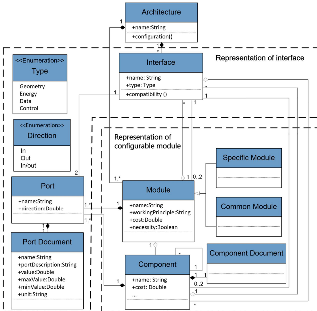
Fig. 2 Representation of template model in UML class diagram
