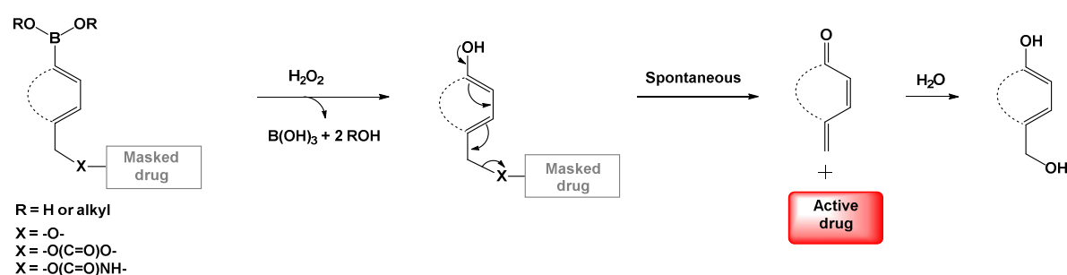
Scheme 1. Conversion of boron-containing prodrug into active drug.
