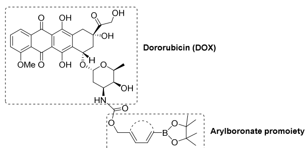
Figure 1. General structure of the arylboronate prodrugs of doxorubicin.
