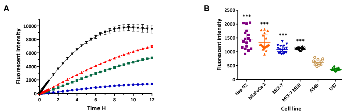
Figure 2. (A) Coumarin release from the arylboronate profluorescent probe 3 in presence of H 2 O 2 (▼ 50 eq., ▲ 10 eq., ◻ 5 eq. and ● 1eq.). (B) Investigation of the capacity of ROS production by cell lines (*statistically significant difference compared to U87 cell line with p < 0.0001 ).
