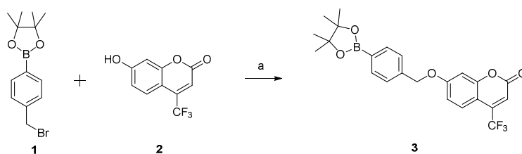
Scheme 2. Synthesis of the arylboronate profluorescent probe 3 . Reagents and conditions: (a) Cs 2 CO 3 , DMF, r.t., 4h.
