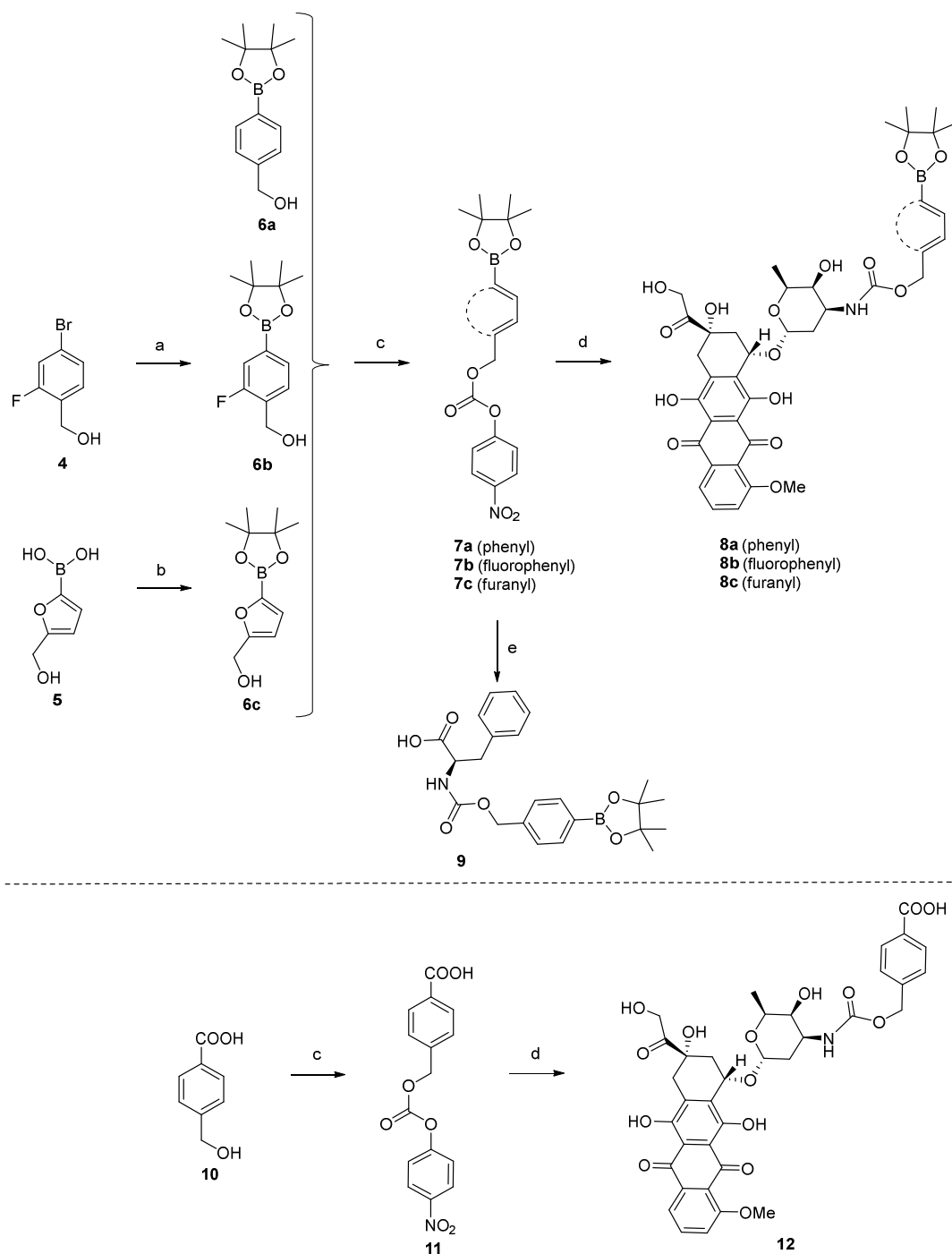
Scheme 3. Synthesis of boronate prodrugs and controls. Reagents and conditions: (a) AcOK, Pd(dppf)Cl 2 ·CH 2 Cl 2 , B 2 (Pin) 2 , DMF, 80°C; (b) pinacol, THF, 40°C; (c) 4-nitrophenyl chloroformate, base, DCM, 0°C to r.t.; (d) DOX·HCl, HOBt, Et 3 N, DMF, r.t.; (e) phenylalanine, HOBt, Et 3 N, DMF, r.t.
