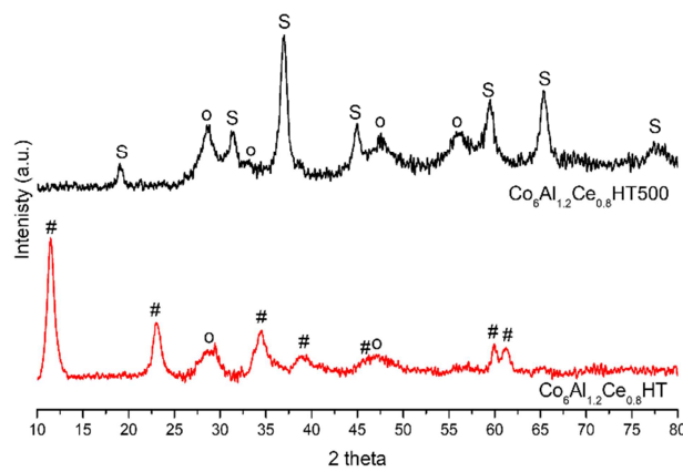
Figure 1 XRD patterns for \text{Co}_6\text{Al}_{1.2}\text{Ce}_{0.8}\text{HT} and \text{Co}_6\text{Al}_{1.2}\text{Ce}_{0.8}\text{HT500} samples (#: \text{Co}_6\text{Al}_2(\text{OH})_{16}\text{CO}_3 \cdot 4\text{H}_2\text{O} , S: \text{Co}_3\text{O}_4 , \text{CoAl}_2\text{O}_4 or \text{Co}_2\text{AlO}_4 , o: \text{CeO}_2 )
