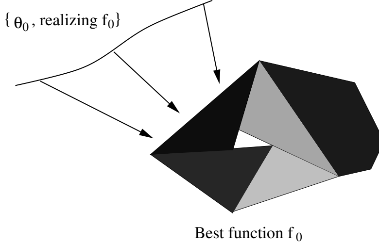
Figure 2: Set of parameters realizing the best function f_0 .
