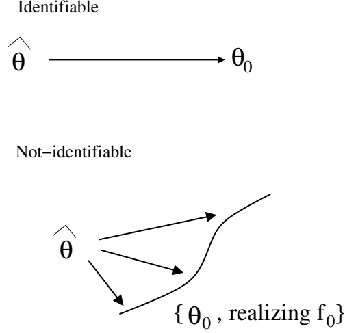
Figure 1: Set of possible paths for the estimated parameter vector \hat{\theta} .
