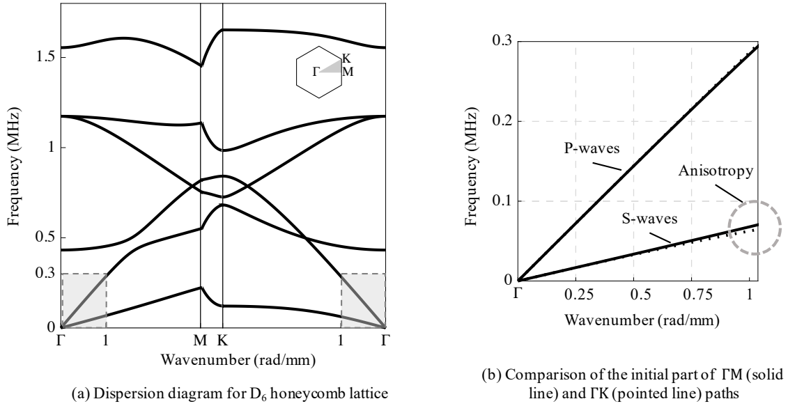
Figure 2: Global (a) and local (b) picture of the dispersion diagram for a hexagonal lattice.
