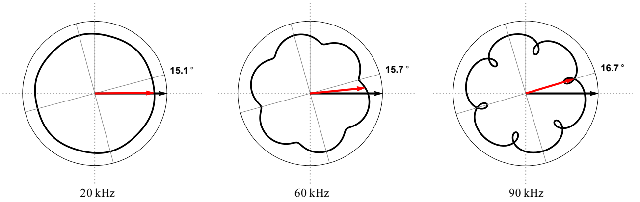
Figure 12: Polar plots of the normalised Poynting vector (red arrow, colors online) corresponding to a wave propagating towards direction \xi indicated by the black arrow.
