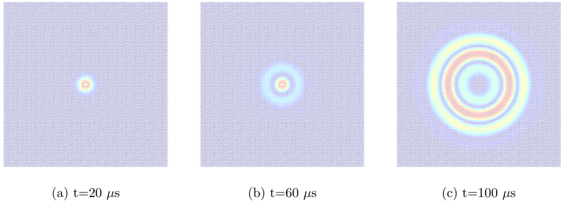
Figure 3: Snapshots of a shear pulse at low frequency (20 Hz) for the honeycomb model ( \eta \ll 1 ). The norm of the displacement is displayed, arbitrary units are used.
