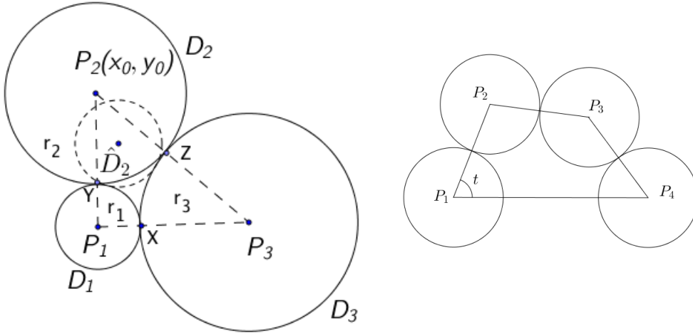
FIGURE 6. Proof of Lemma 19: initial step (left) and induction step (right)
