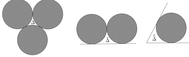
FIGURE 1. The three types of empty regions: \Delta, \widehat{\Delta}, \widehat{\widehat{\Delta}}
