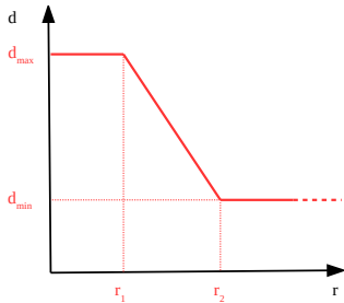
Figure 8: Target density as a function of the distance to the crack front.
