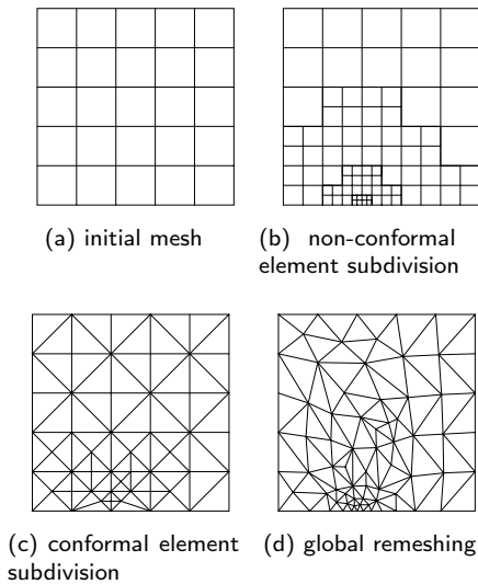
Figure 2: h -refinement
