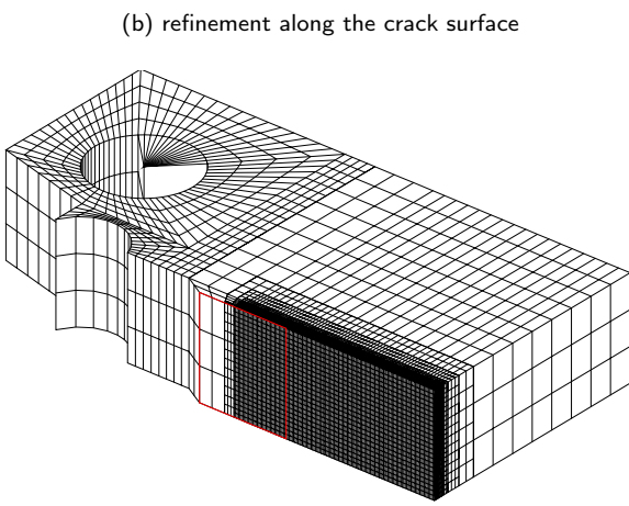
Figure 22: Meshes at the propagation step 25 for different refinement strategies
