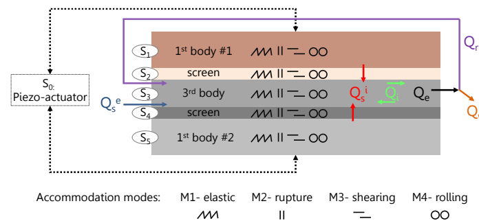
Fig. 1. 3 rd body formalism. The tribological triplet is composed of a mechanism, the rubbing 1 st bodies and the 3 rd body particles. Resulting tribological circuit - described in nomenclature and used in this work - is characterized by (i) solid particle flows and (ii) velocity accommodation mechanisms decomposed in location sites S_i and accommodation modes M_j [14].
