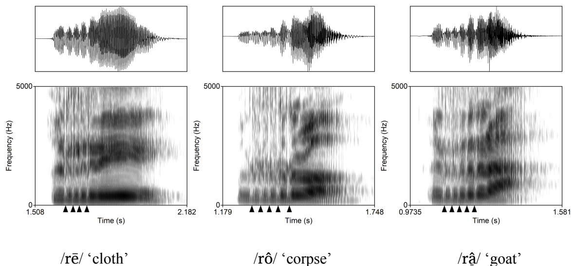
Figure 9. Waveforms and spectrograms for the words /r\bar{e}/ 'cloth', /r\hat{o}/ 'corpse', and /r\hat{a}/ 'goat' with arrows indicating contacts between the tip of the tongue and the roof of the mouth.
