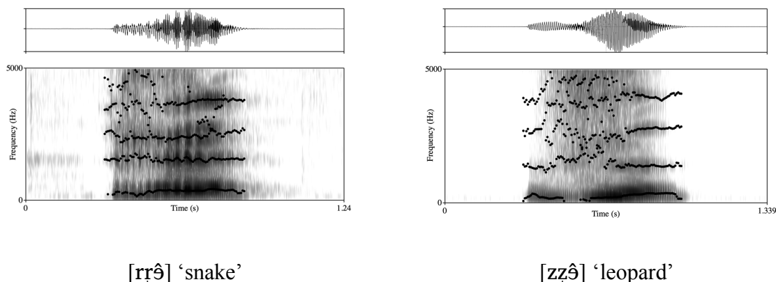
Figure 10. Waveforms, spectrograms, and formant tracks for the words [rɾə̃] ‘snake’ and [zʒə̃] ‘leopard’
