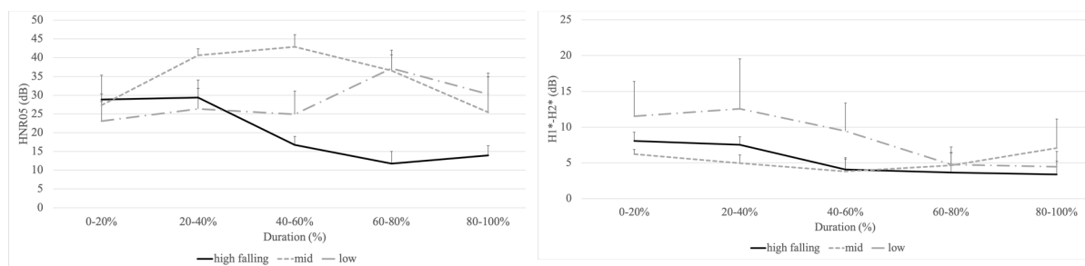
Figure 15. Time courses of HNR05 (dB) (left) and H1*-H2* (dB) (right) in two minimal triplets for tone: (i) /ɲê/ ‘fire’, /ɲē/ ‘to sleep’, /ɲè/ ‘mountain god’, and (ii) /nô/ ‘inside’, /nō/ ‘heaven, sky’, /nò/ ‘to exist’ (with three repetitions per word, a total of 18 tokens). The x-axis represents vowel duration divided into five regions: 0-20%, 20-40%, 40-60%, 60-80%, 80-100%. High falling tone in black solid line, mid tone in light gray dotted line, low tone in gray dashed line.
