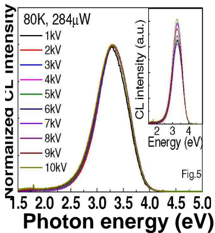
Fig.5 Depth-resolved CL spectra showing a self-trapped excitation peak, independent of sampling depth.
