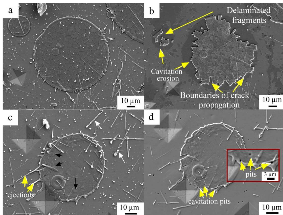
Figure 5: Morphology of single splats for (a) YSZ without cavitation, (b) YSZ after cavitation for 2 min, (c) 304SS without cavitation, and (d) 304SS after cavitation for 2 min
