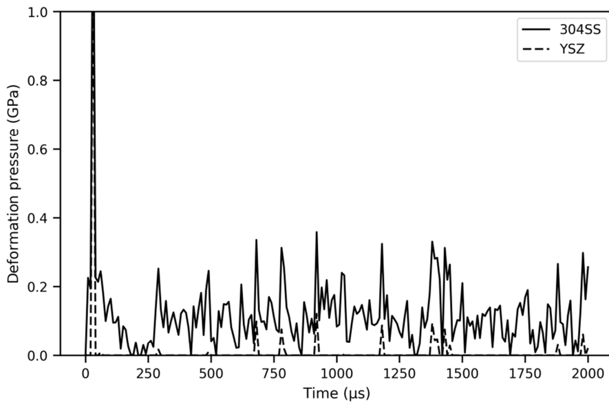
Figure 8: Transient evolution of mean deformation pressures for 304 and YSZ
