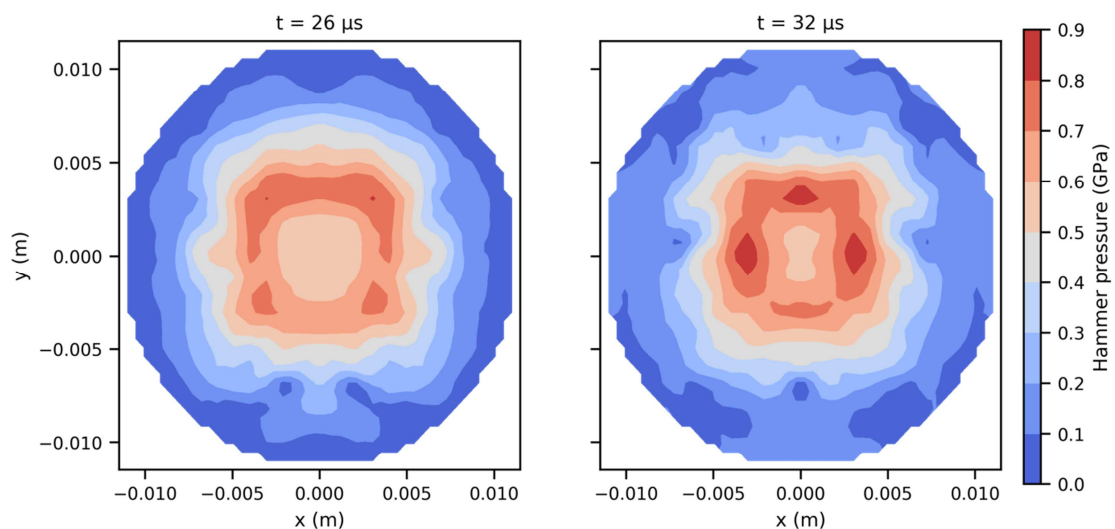
Figure 6: Hammer pressure contour on the surface of specimen at t = 26 μs and t = 32 μs
