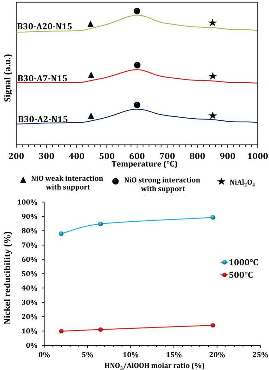
Figure 7: Influence of the HNO 3 amount on the nickel species and reducibility
