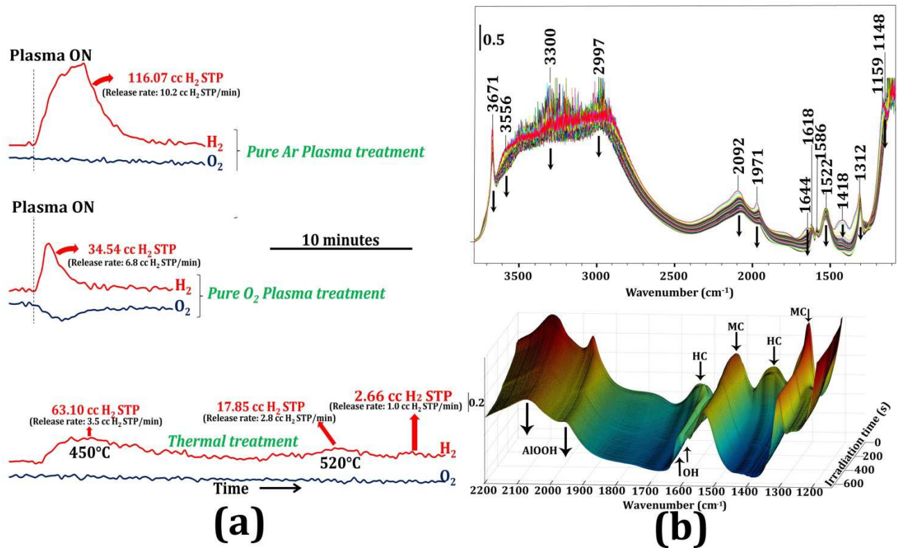
Figure 3: Mass spectrometry signal of H 2 (red) and O 2 (blue) during plasma and thermal treatment of boehmite (a); Operando analysis of plasma treatment on boehmite (b)
