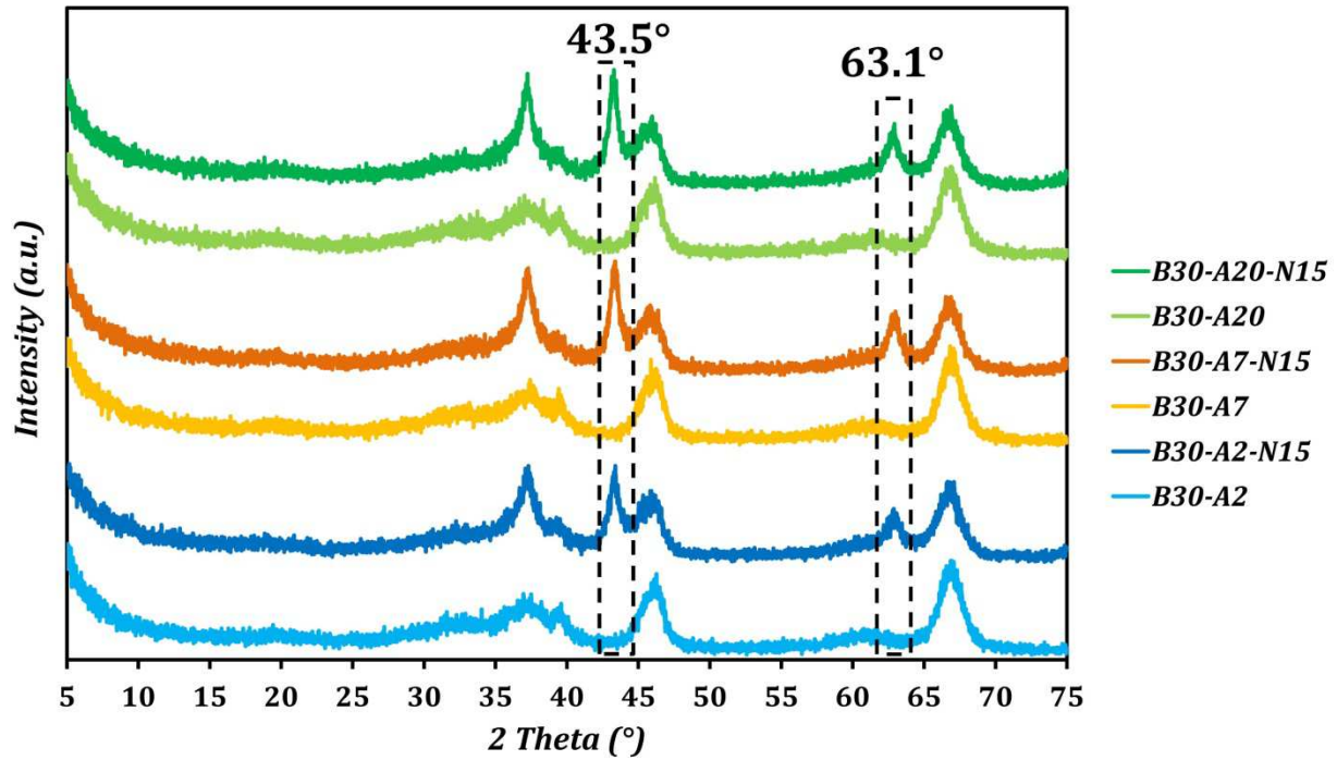
Figure S2: XRD patterns of Ni-Alumina porous extrudates
