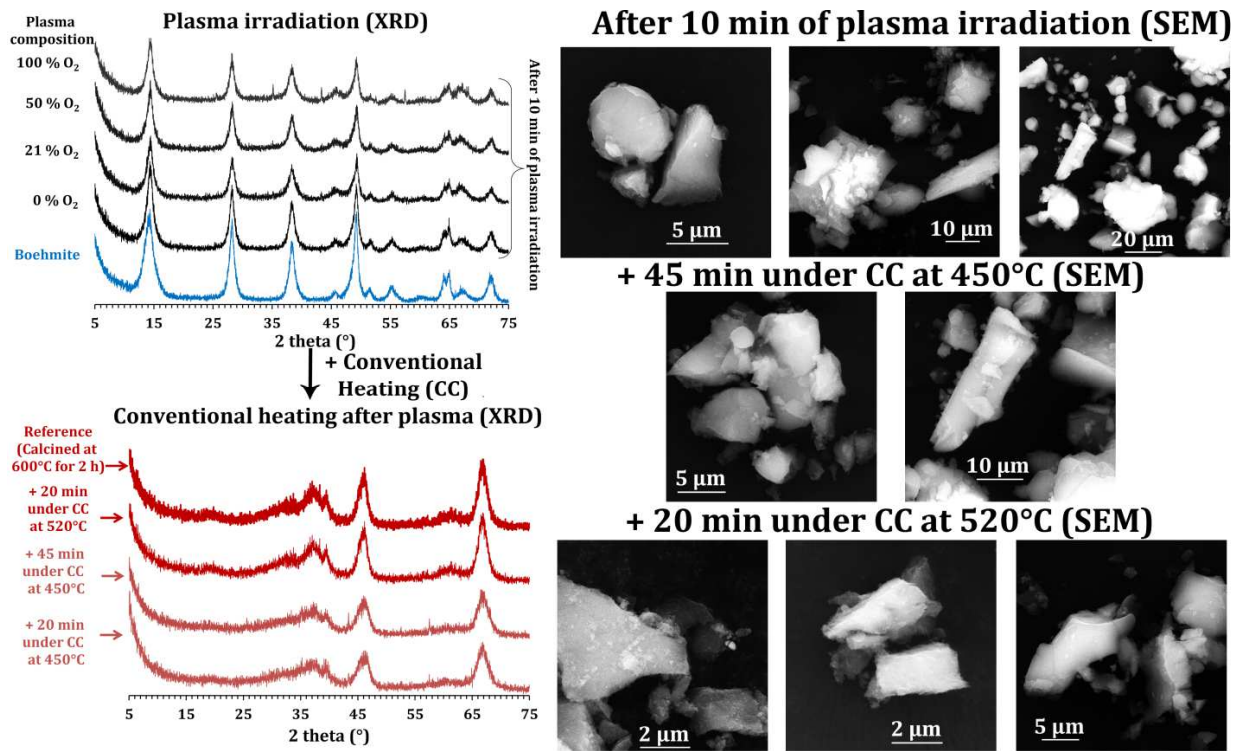
Figure 4: Thermal post-treatment study after plasma irradiation for successfully transform \gamma\text{-AlOOH} into \gamma\text{-Al}_2\text{O}_3
