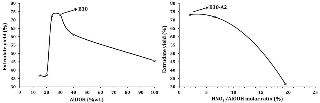
Figure 6: Optimization of alumina porous extrudates preparation
