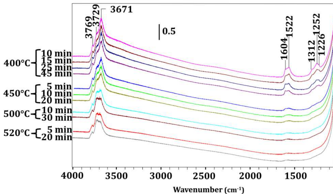
Figure 5: FTIR operando analysis of post-thermal treatment at different temperatures
