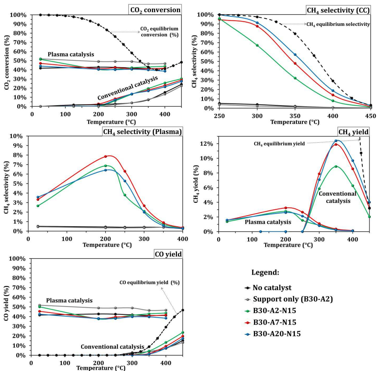
Figure 10: CO 2 conversion, CH 4 selectivity and yield of CO 2 hydrogenation under plasma and conventional heating. Under classical catalysis, catalysts were only active from 200°C and CO 2 conversion was favored with temperature. No significant differences were observed between the three Ni-
